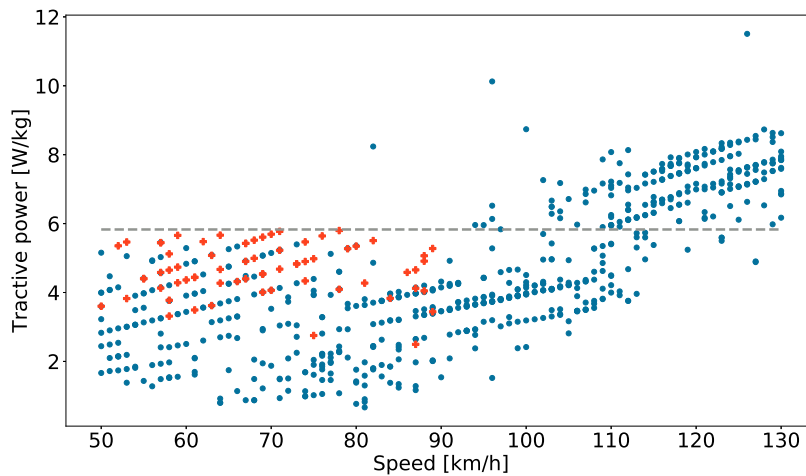
Fig. 9. Tractive power diagram of the initial acceleration phase of the 67 considered speed profiles.
