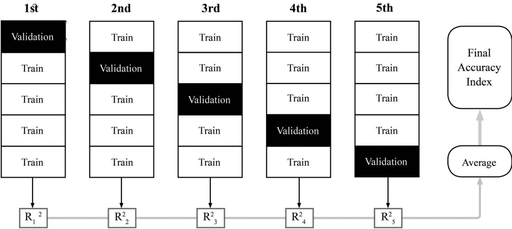
Figure 5. Cross-validation.
