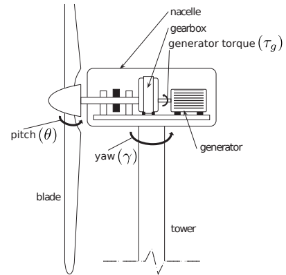
Fig. 3. Horizontal-axis wind turbine with labeled main components and control variables. Figure adapted from [13].
