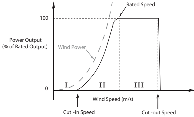
Fig. 4. Typical wind turbine power curve. Figure adapted from [15].
