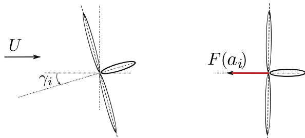
Fig. 7. A schematic representation of wind farm actuators typically used in simulations. The thrust force, F(a_i) , is determined by the axial induction a_i of turbine i .
