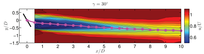
Fig. 5. A time-averaged, stream-wise wind velocity contour plot at hub height obtained from wind tunnel data. The center of the wake is shown in filled magenta circles. Figure taken from [29].
