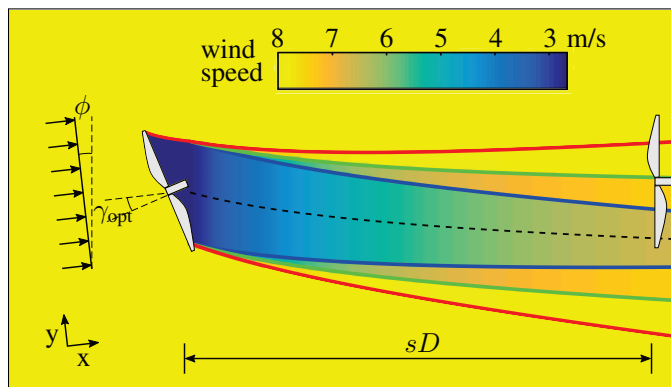
Fig. 9. An illustration of wake redirection control with inflow angle \phi and a second turbine placed s rotor diameters D downstream of the first turbine. Figure taken from [36].
