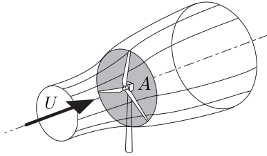
Fig. 2. Flow with velocity U [m/s] through a rotor disk with rotor swept area A [m 2 ]. Figure adapted from [12].
