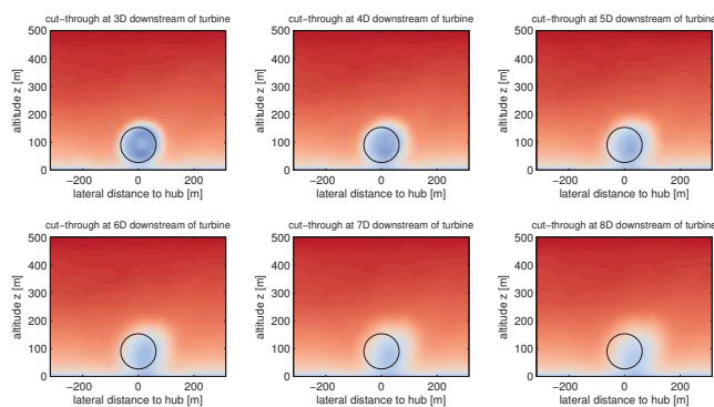
Fig. 8. A cut-through at different distances of a wake from SOWFA data (red colored area contains higher wind velocity than the blue colored area). Figure taken from [9].
