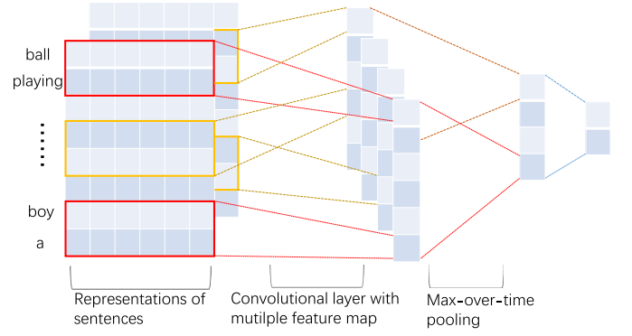
Fig. 4. The convolution process of input sentence in discriminative model.
