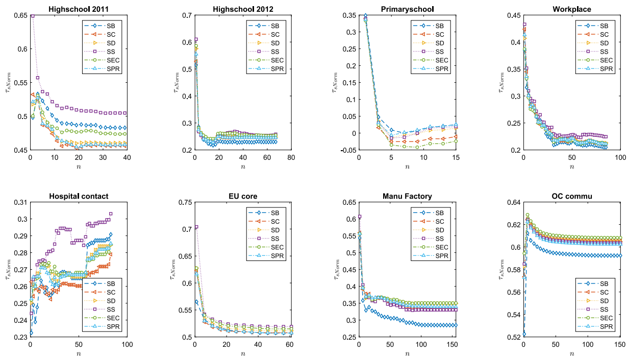
FIG. 10. The evolution of \tau_s^{\text{Norm}} between std-tig-score and R_{\text{norm}} as the gathering depth n increases.
