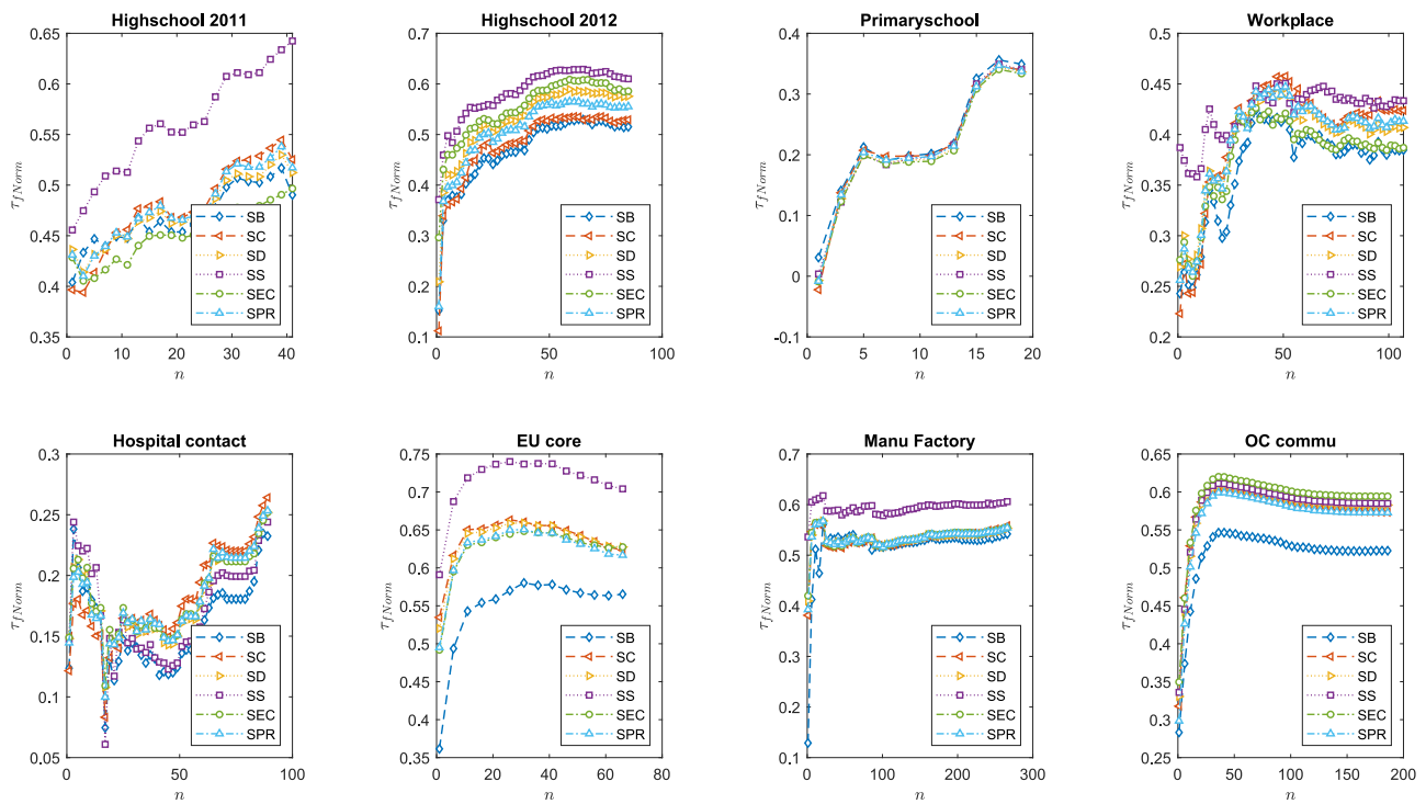
FIG. 9. The evolution of \tau_f^{\text{Norm}} between fad-tig-score and R_{\text{norm}} as the gathering depth n increases.
