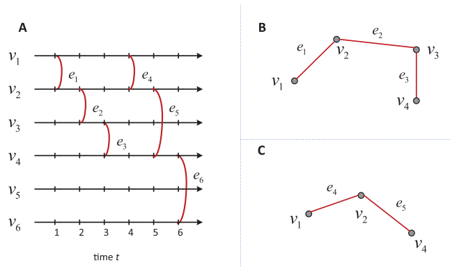
FIG. 1. (a) A schematic representation of a temporal network with nodes \{v_1, v_2, \dots, v_6\} and events \{e_1, e_2, \dots, e_6\} . There are two paths between node v_1 and v_4 . (b) The fastest arrival path between nodes v_1 and v_4 . (c) The temporal shortest path between nodes v_1 and v_4 .
