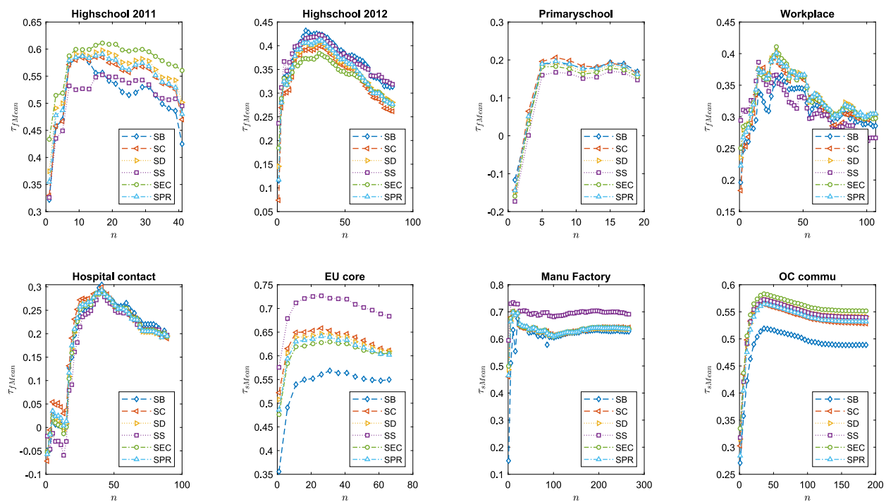
FIG. 14. The evolution of \tau_{fMean} between fad-tig-score and R_{mean} as the gathering depth n increases.
