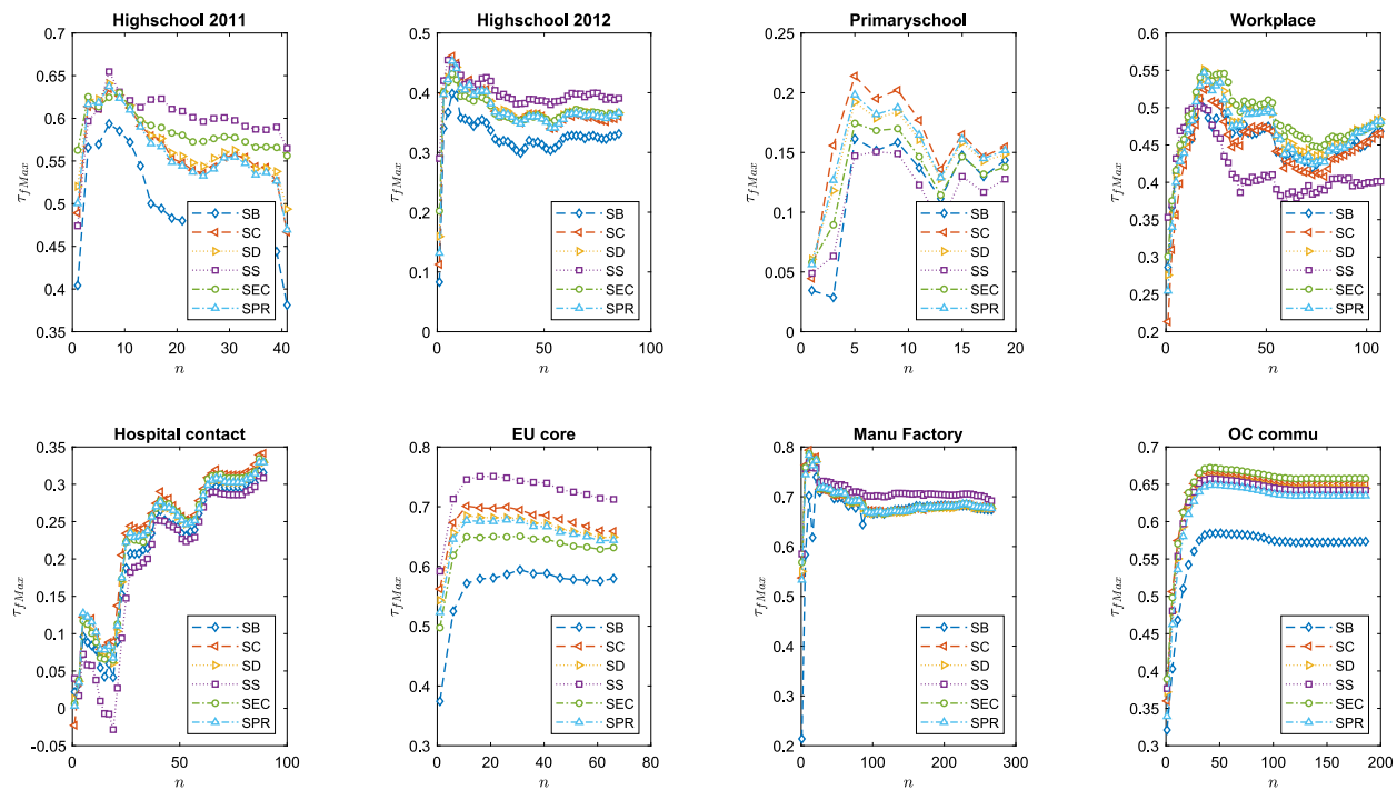
FIG. 13. The evolution of \tau_{fMax} between fad-tig-score and R_{max} as the gathering depth n increases.
