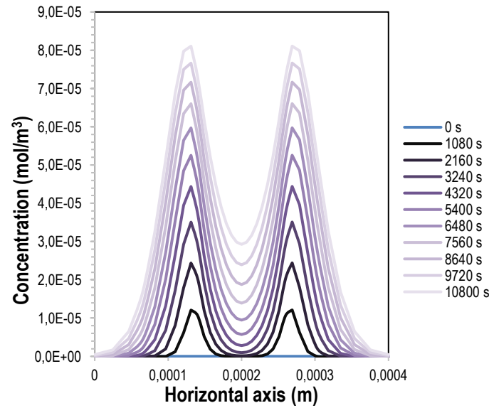
Figure 5. Predicted variation of concentration of dissolved species along the horizontal axis over time.
