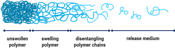
Figure 1. Polymer dissolution process.
