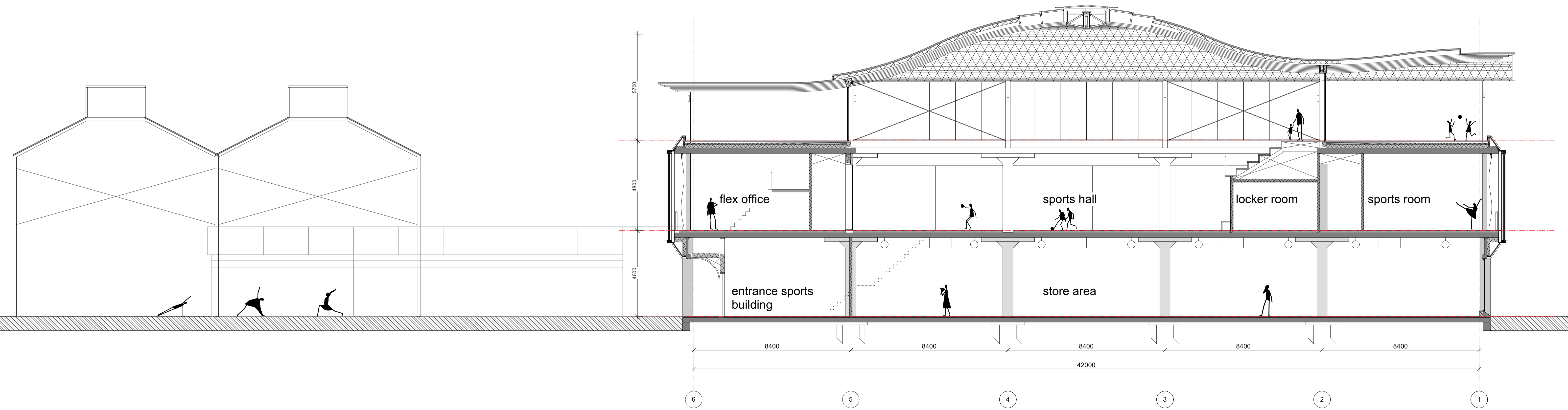
Section BB
