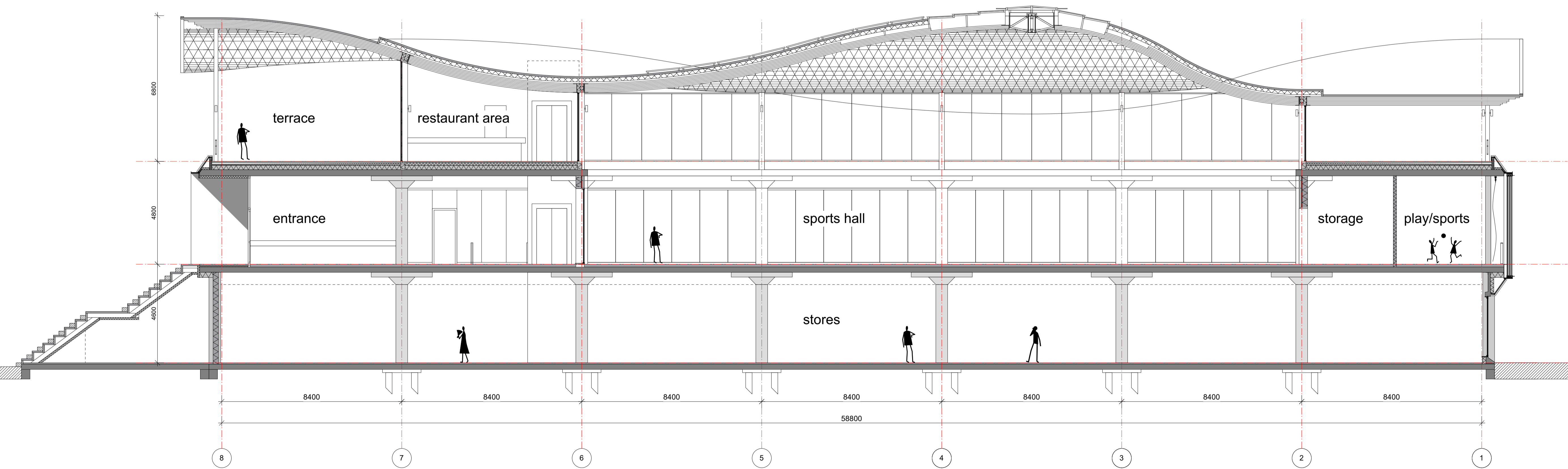
Section AA
