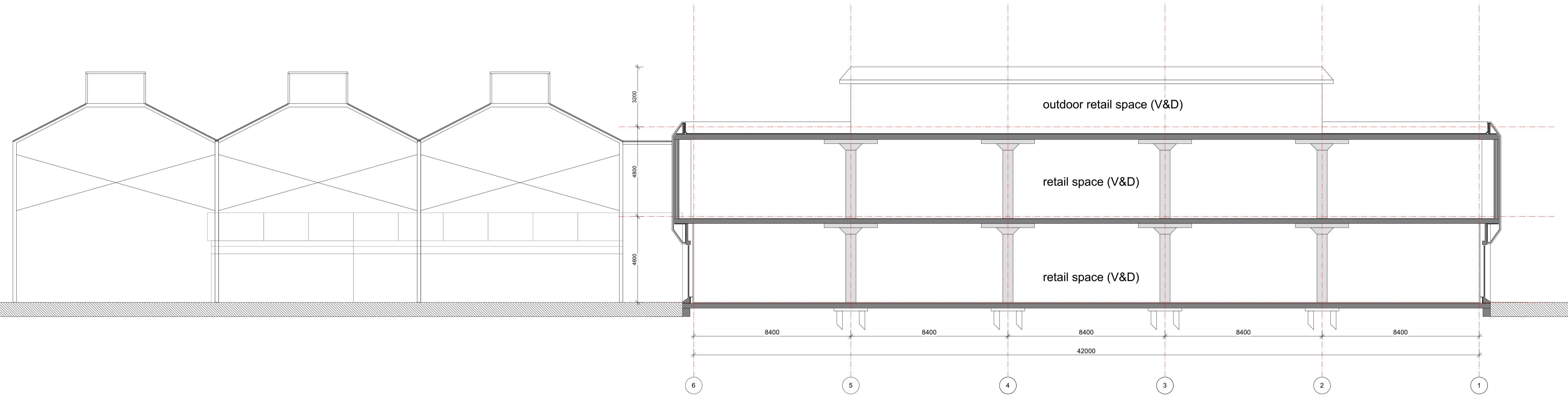
Section BB
