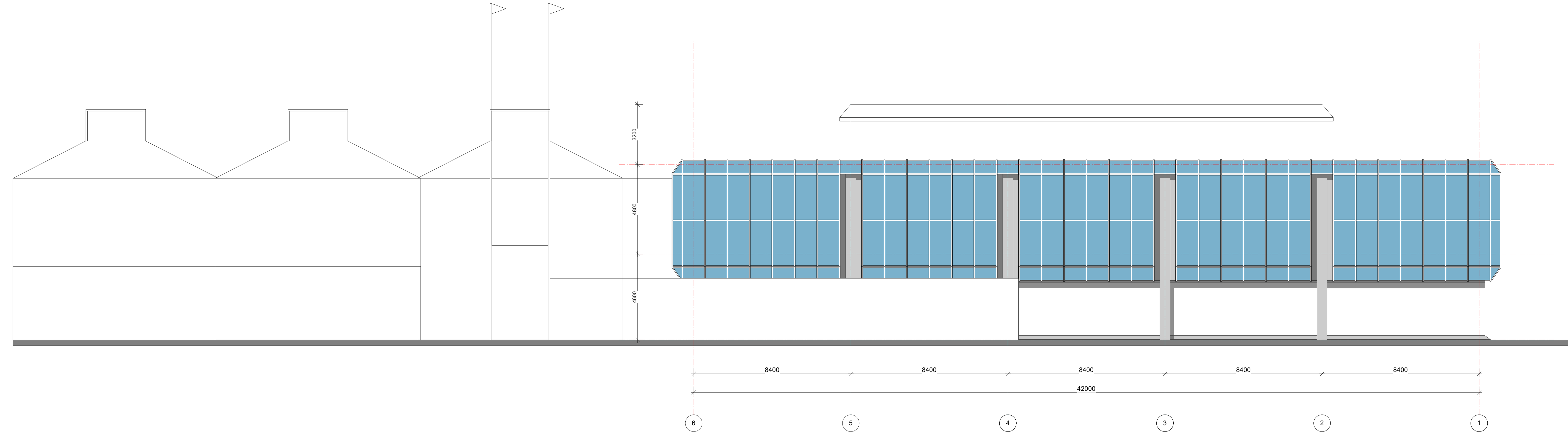
Facade South
