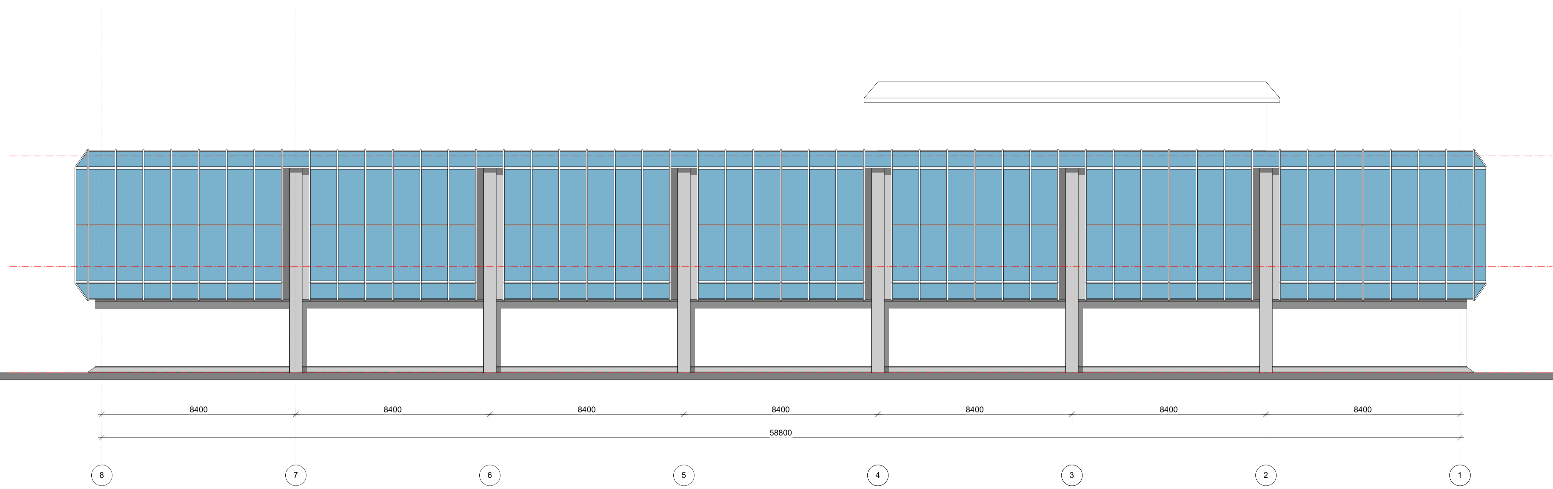
Facade East
