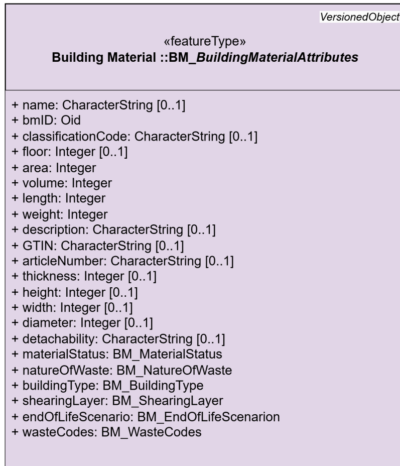
Figure 3.9: Building Material:: BM_BuildingMaterialAttributes
