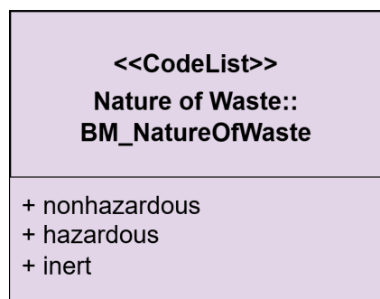
Figure 3.14: Codelist for BM_NatureOfWaste
