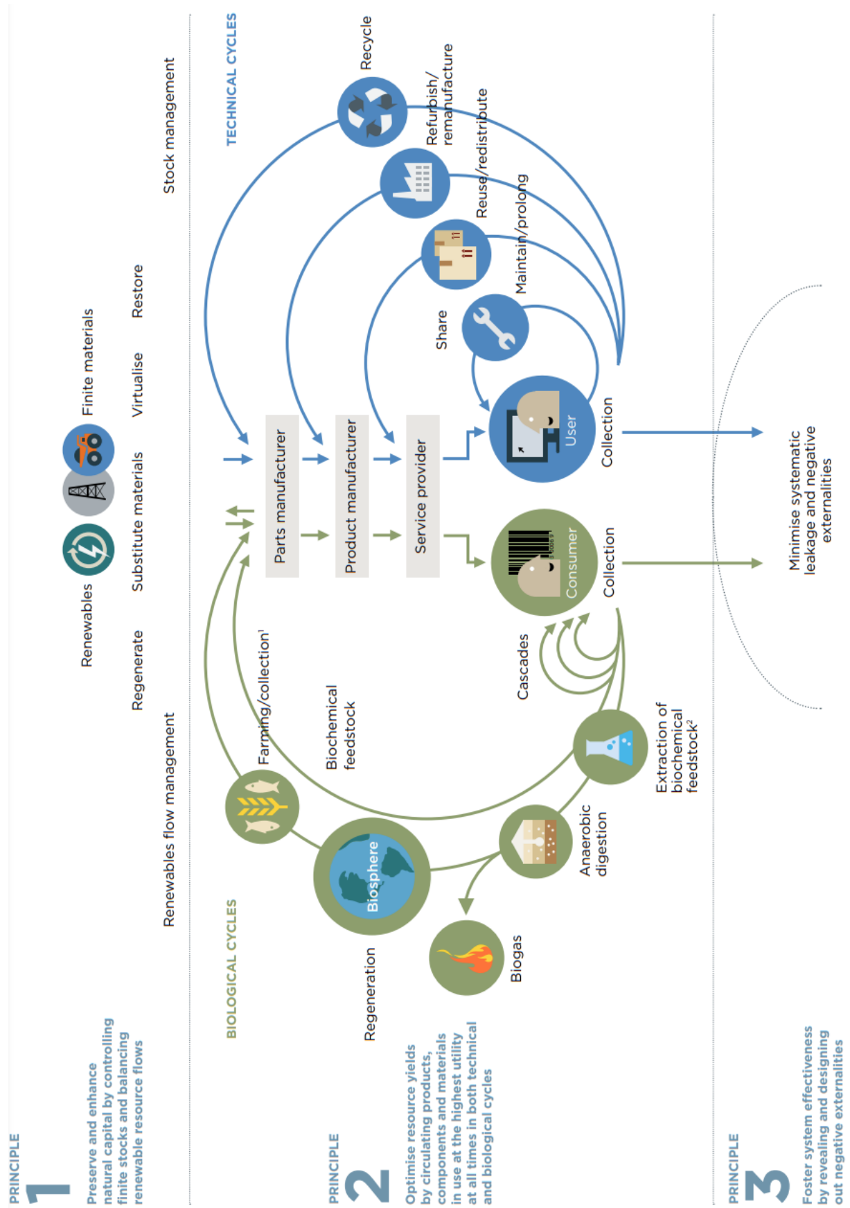
Figure 2.1: Butterfly diagram[MacArthur, 2015]
