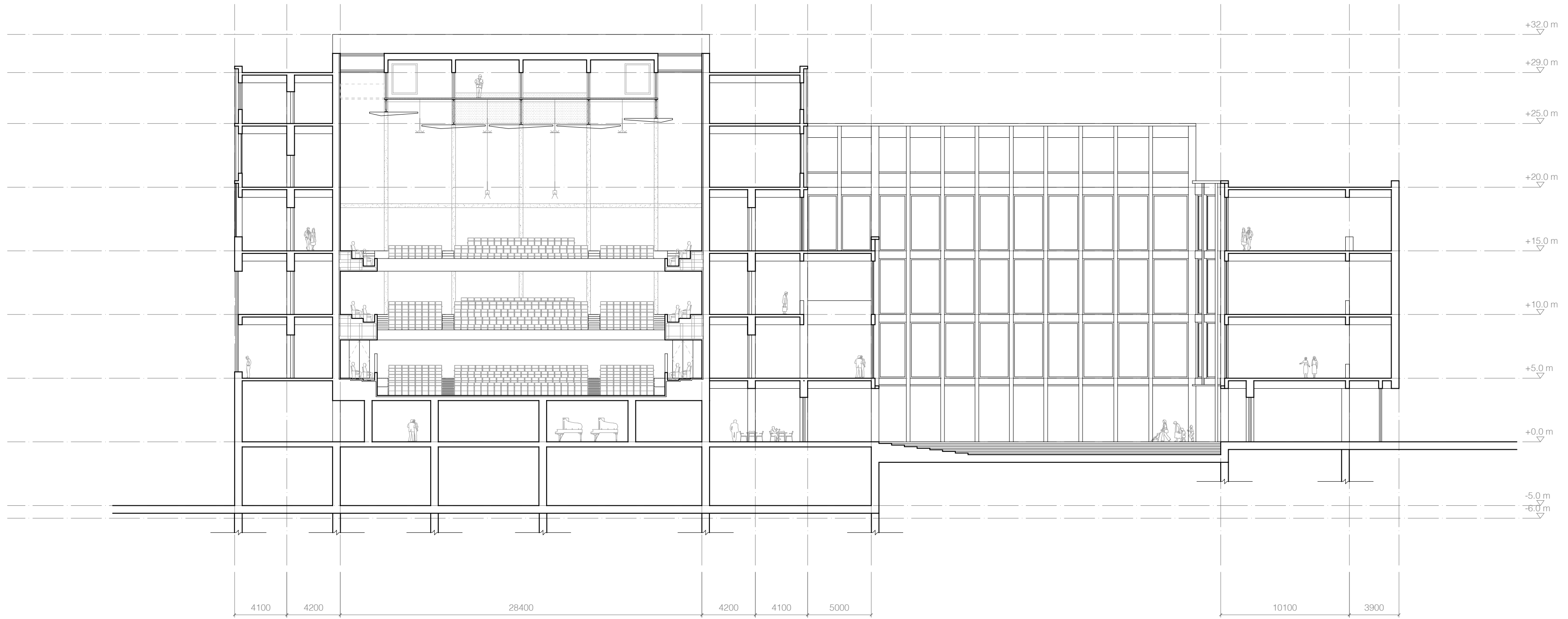
Section AA' 1:250
