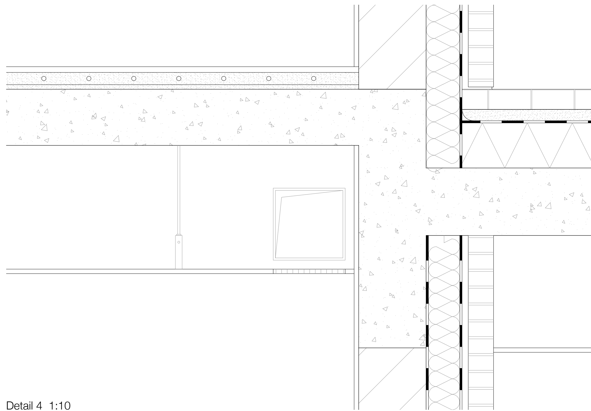
Detail 4 1:10
