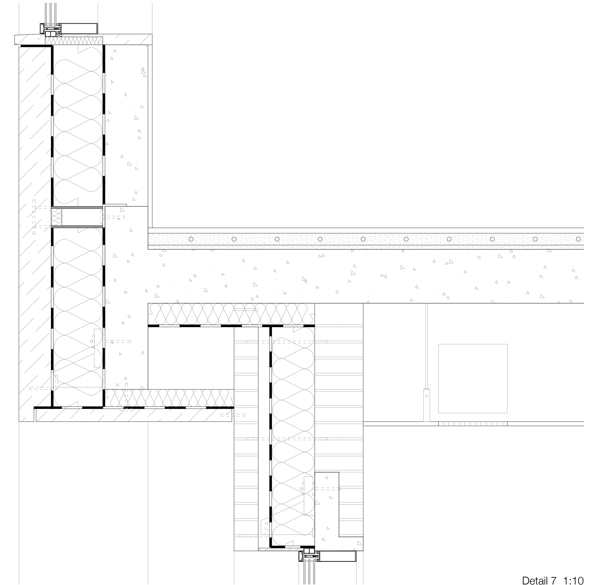
Detail 7 1:10
