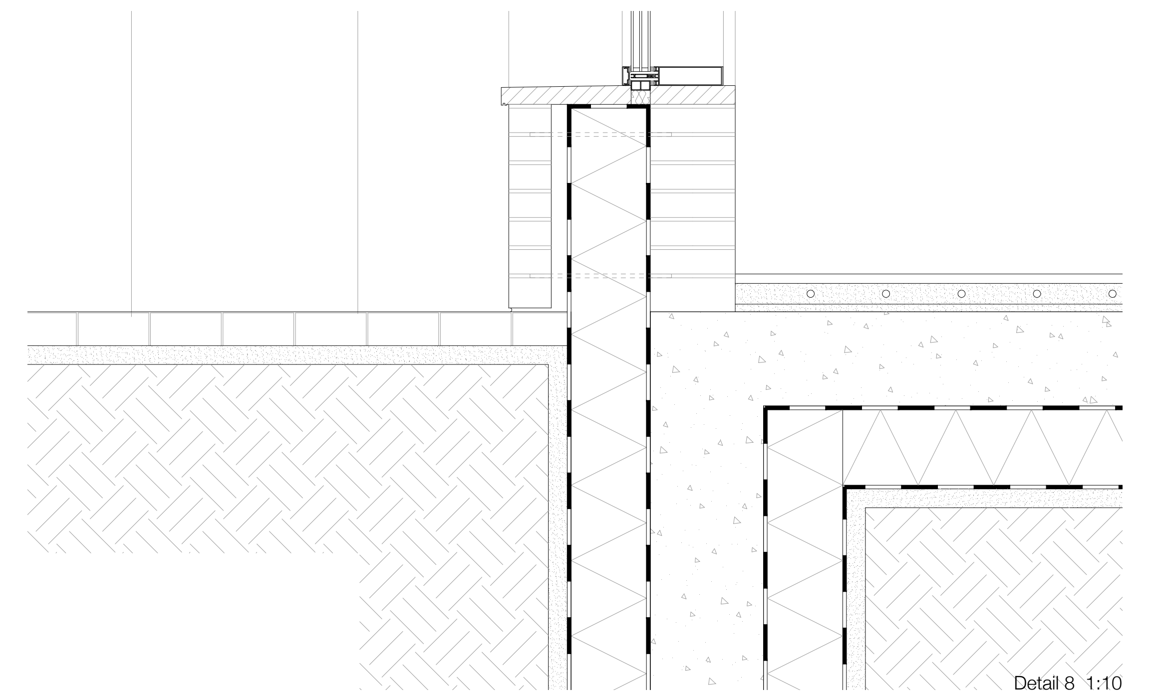
Detail 8 1:10
