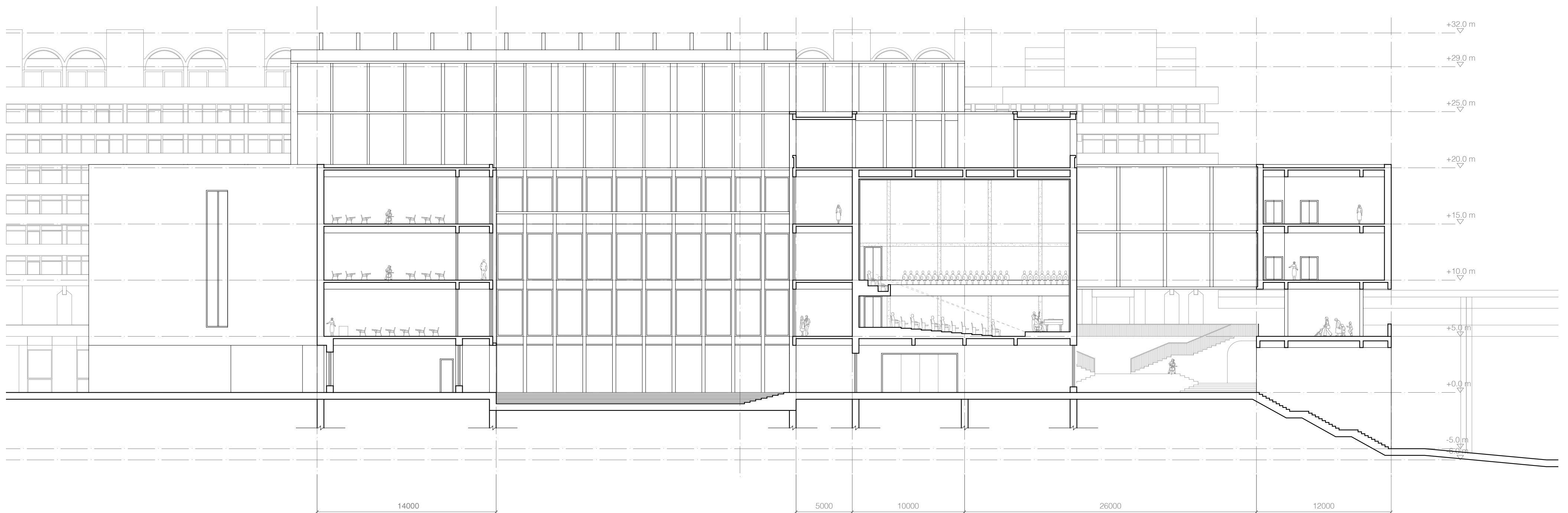
Section CC' 1:250
