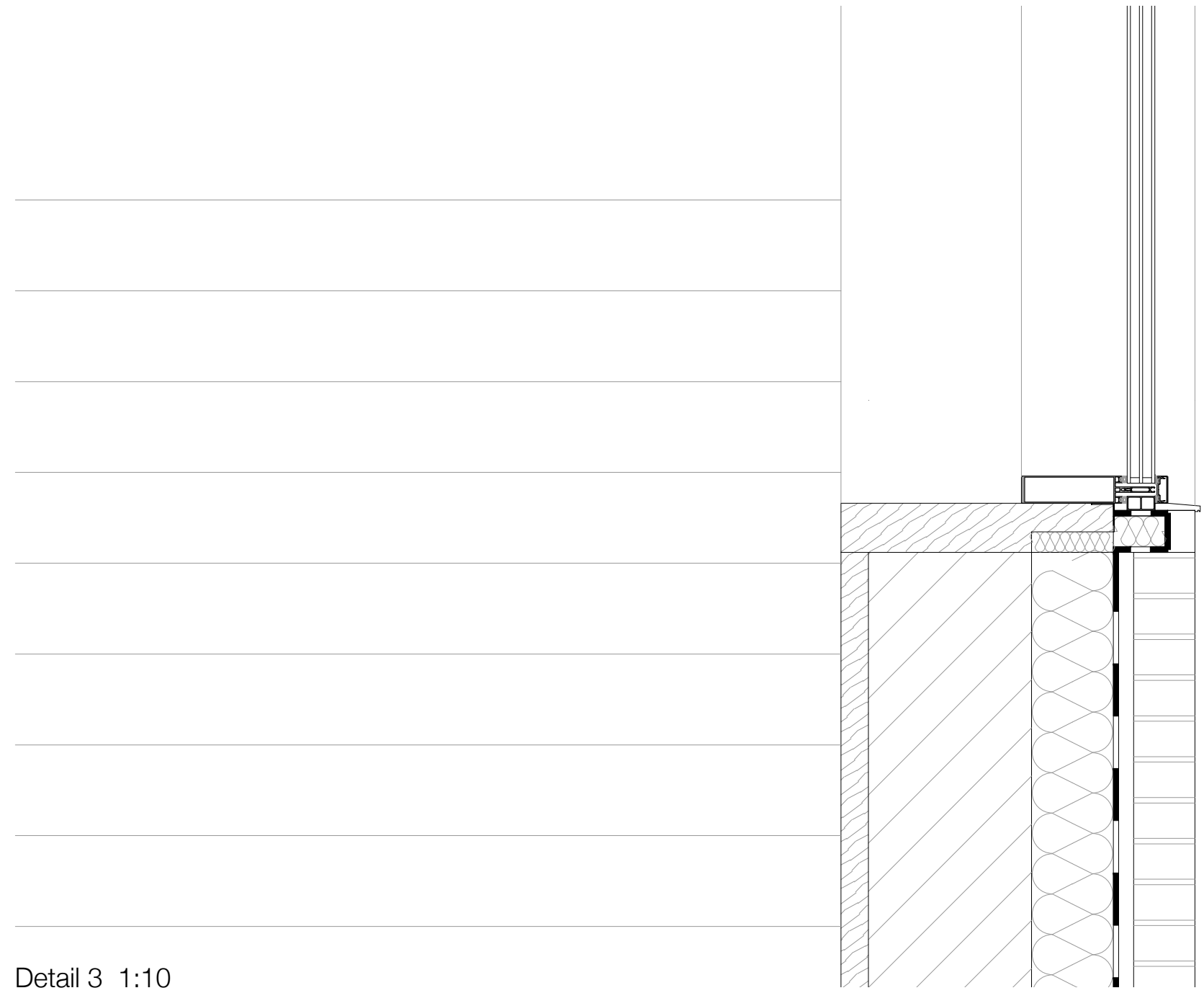
Detail 3 1:10
