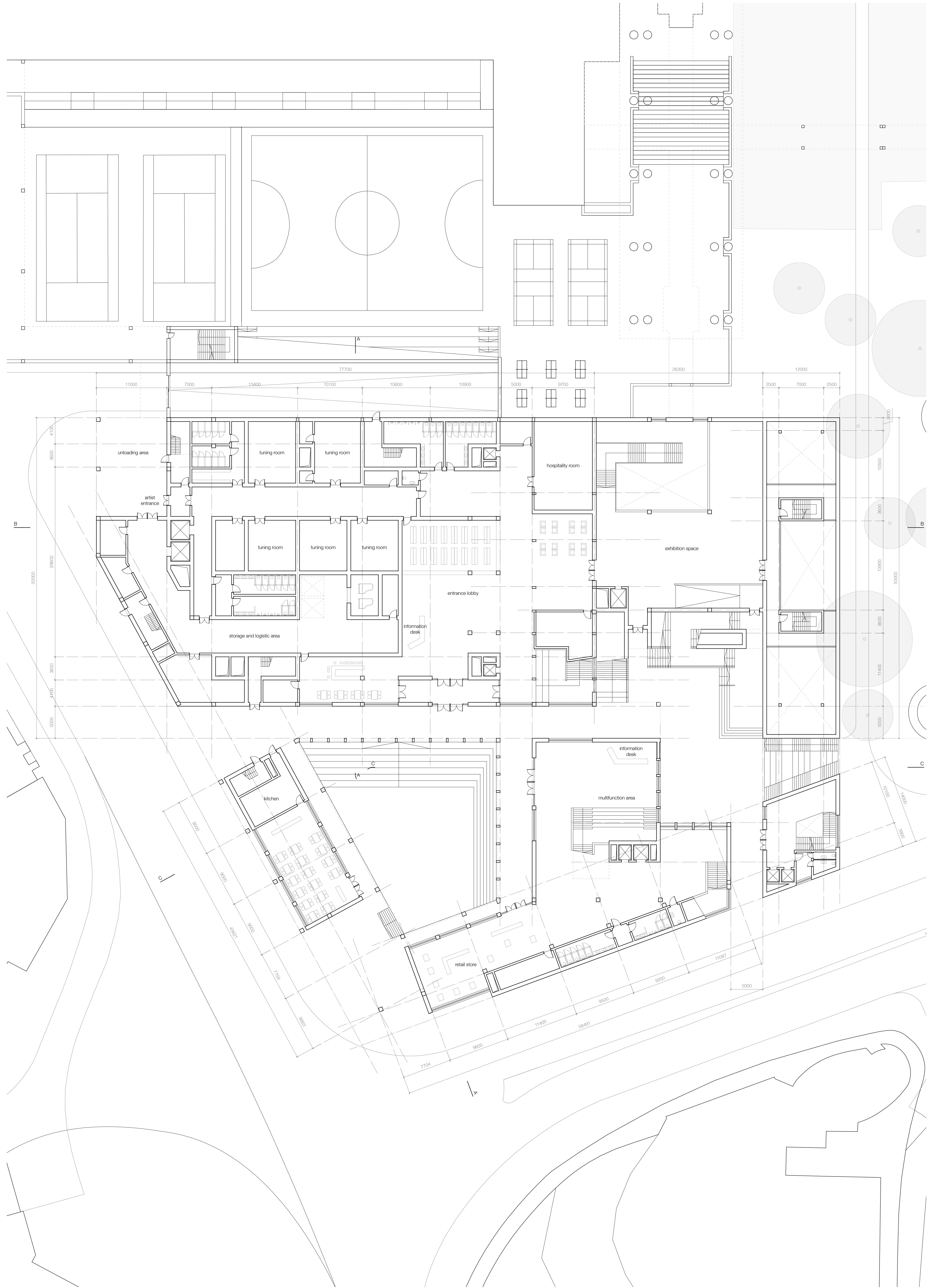
Ground Floor Plan (level +0.00) 1:250
