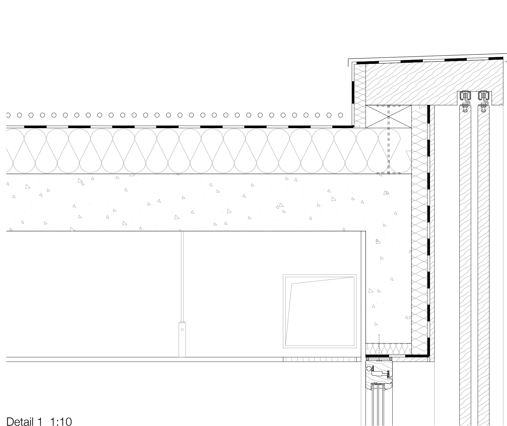
Detail 1 1:10
