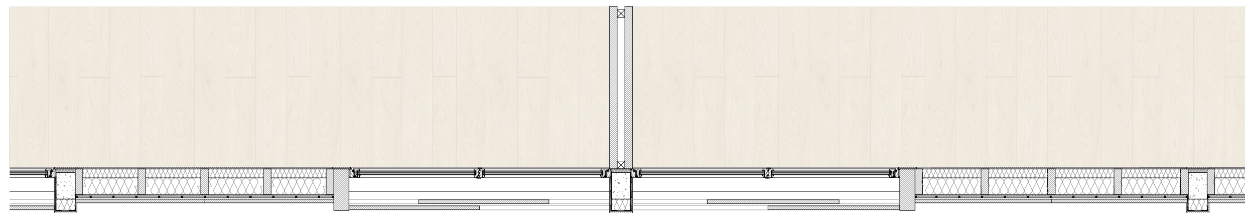
Horizontal section bb 1:50
