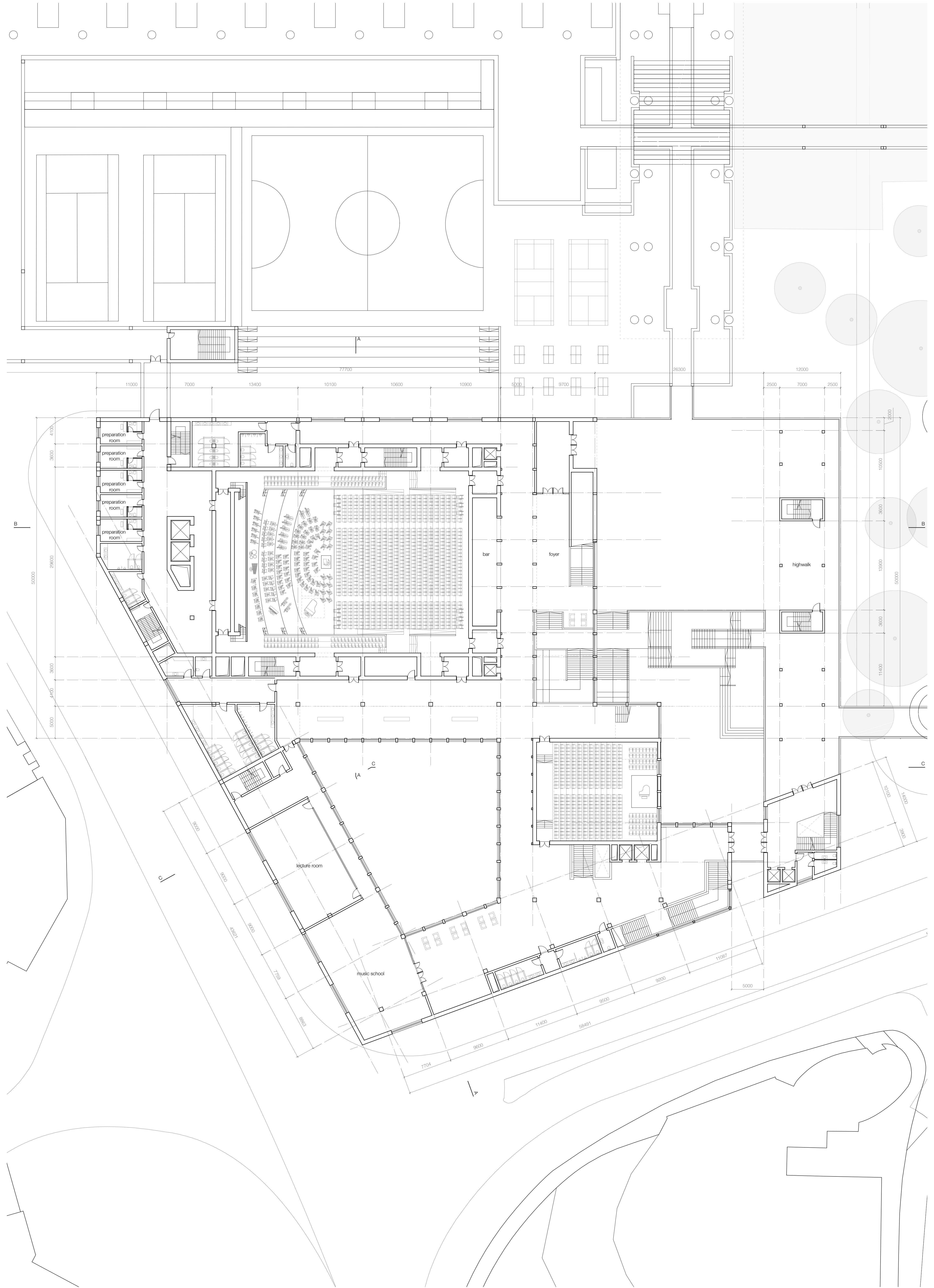
+1 Floor Plan (level +5.00) 1:250
