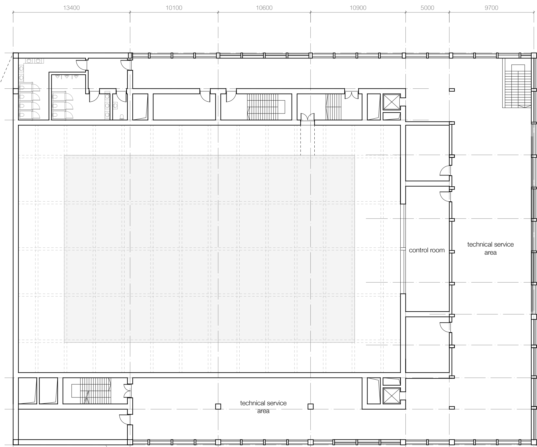
+5 Floor Plan (level +25.00) 1:250
