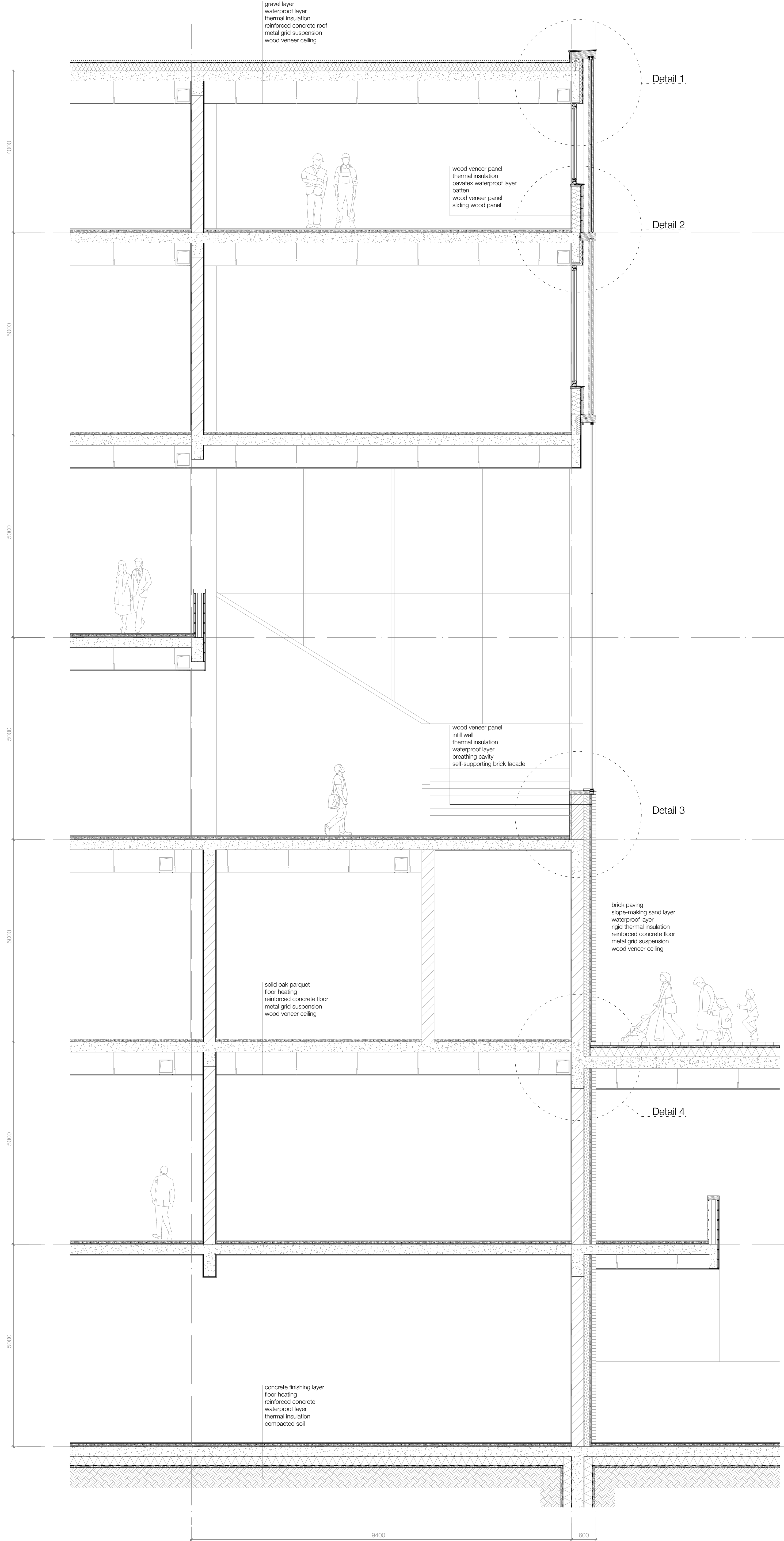
Vertical section cc 1:50
