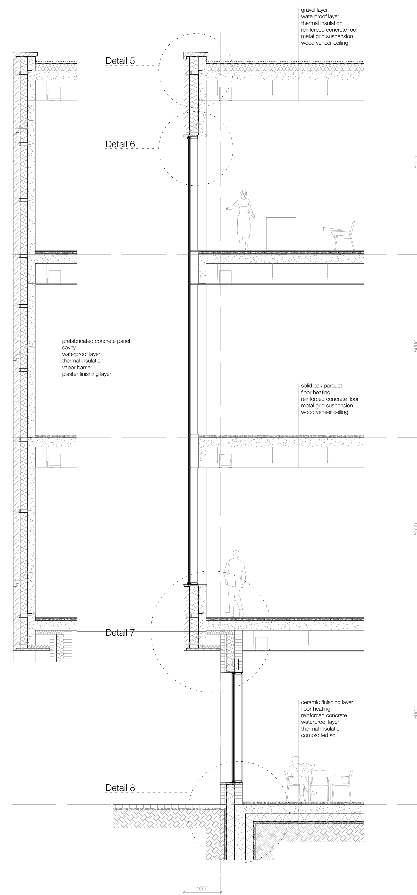
Vertical section ee & ff 1:50
