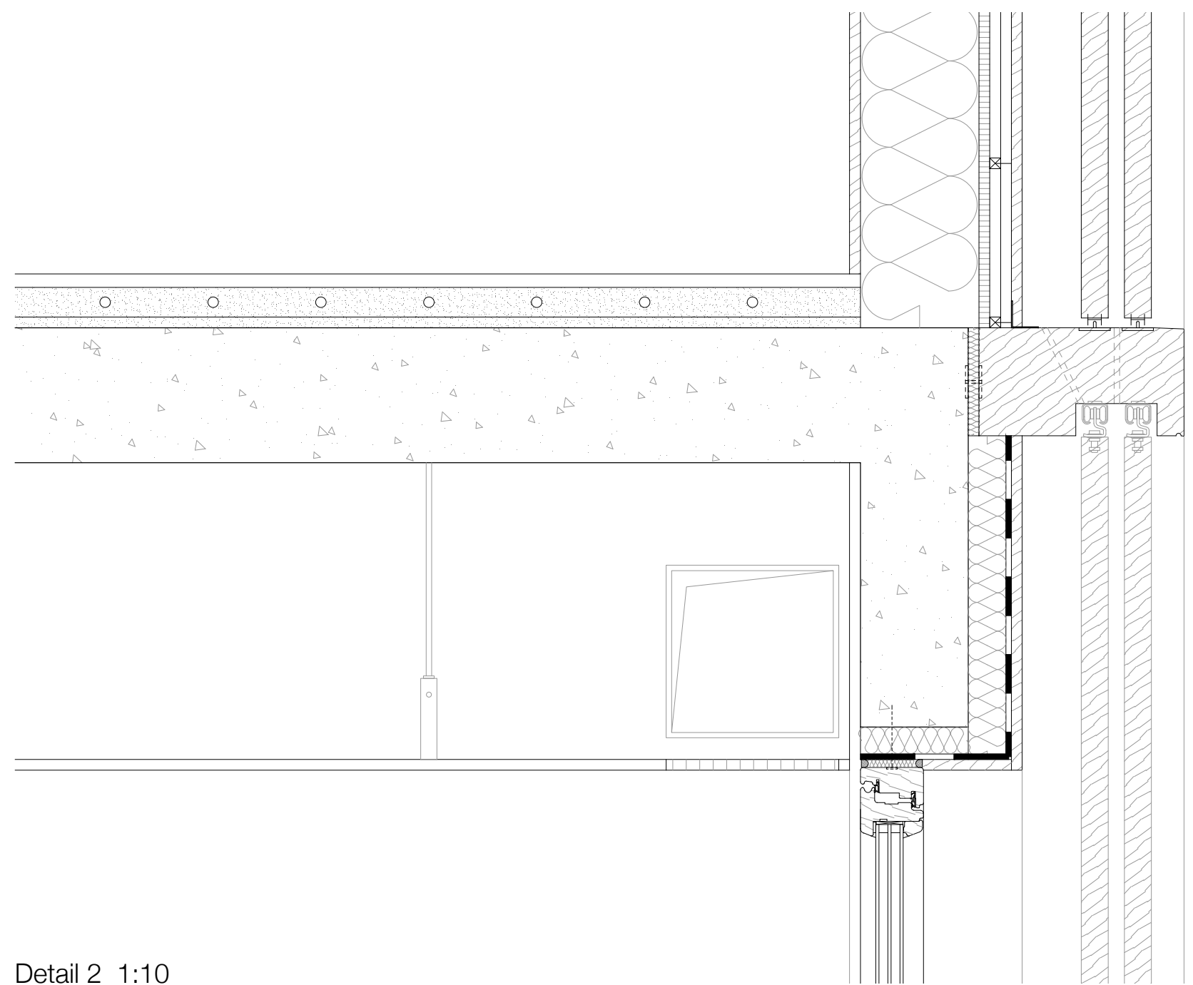
Detail 2 1:10
