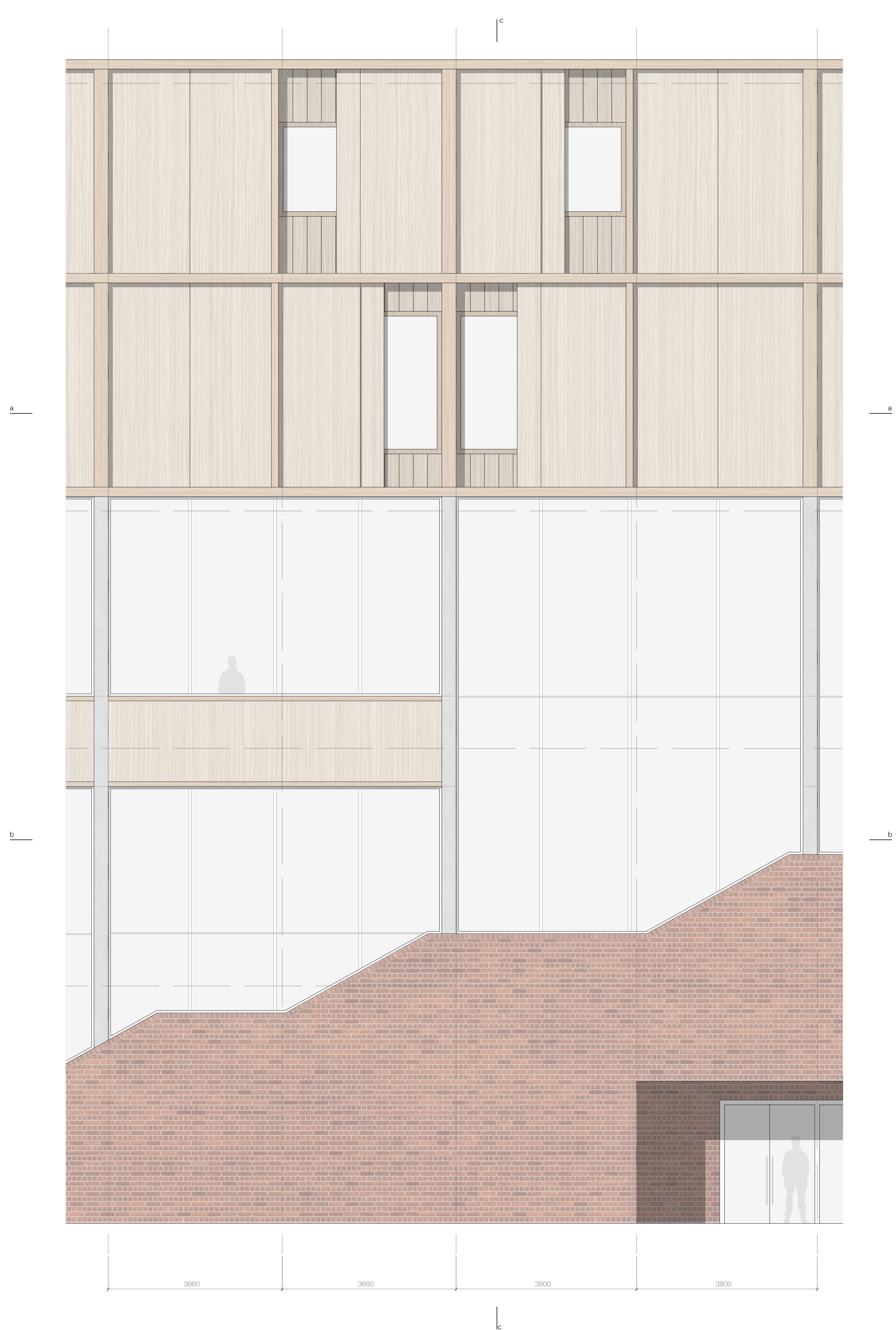
Elevation fragment 1:50
