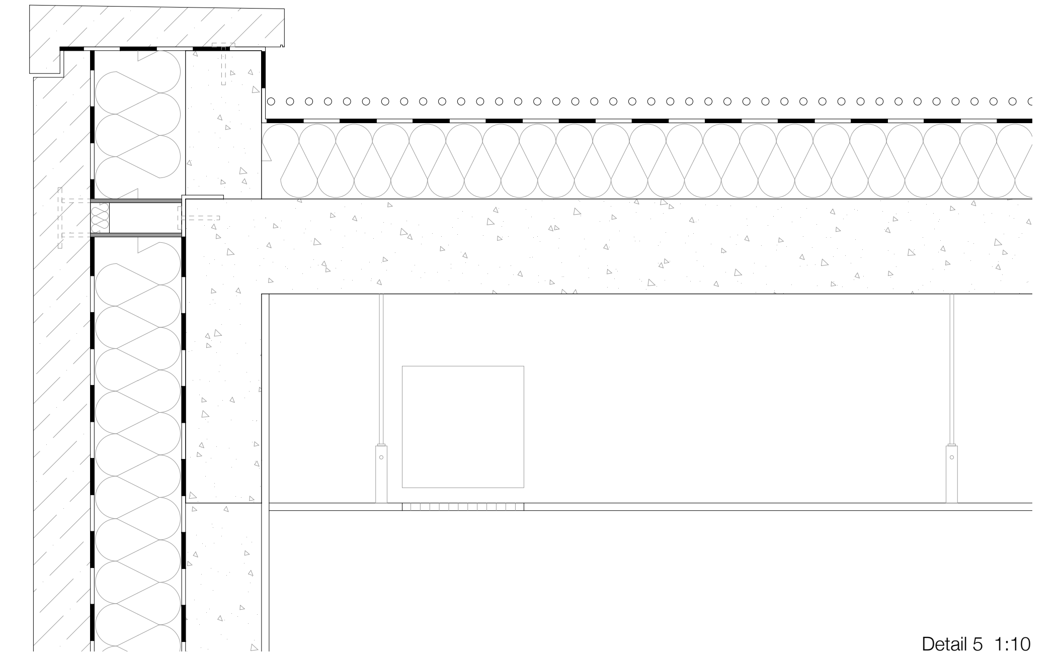
Detail 5 1:10
