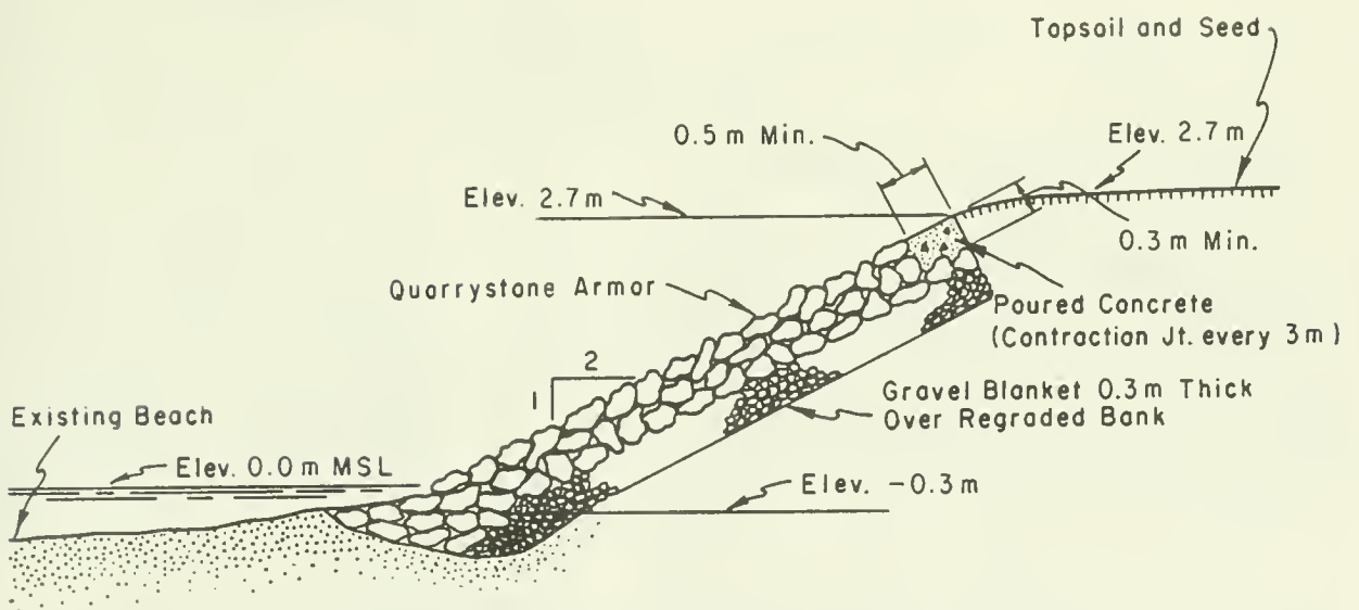
Figure 6-10. Quarrystone revetment.
