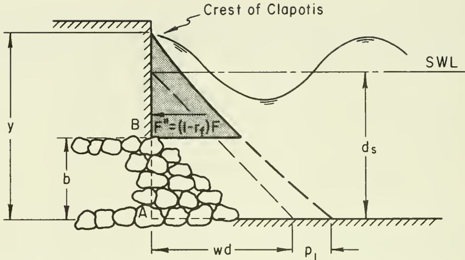
Figure 7-98. Pressure distribution on wall on rubble foundation.
