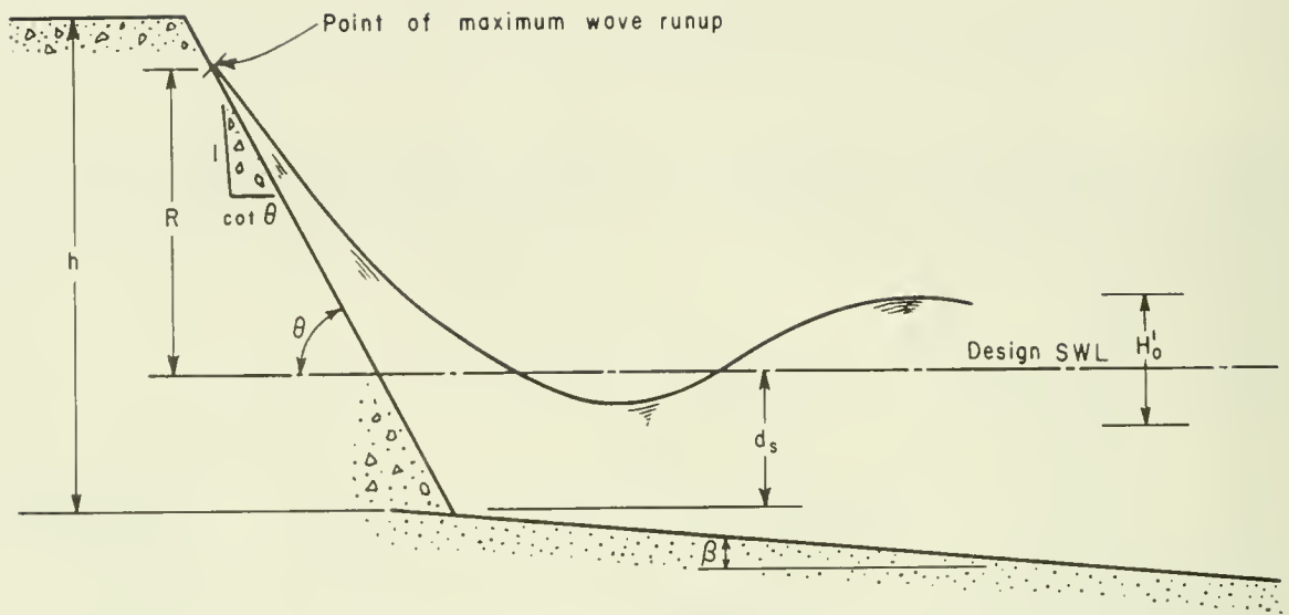
Figure 7-7. Definition sketch: wave runup and overtopping.
