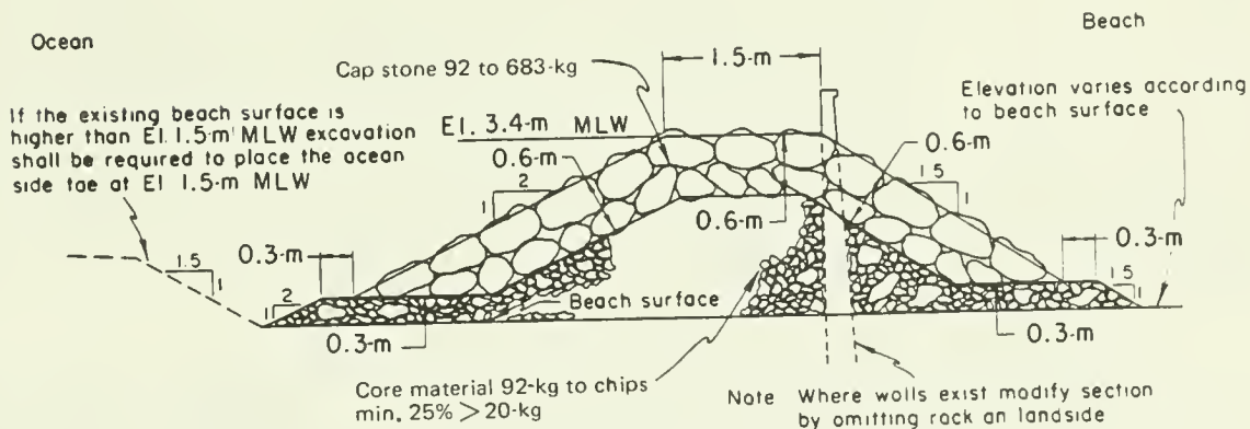
Figure 6-4. Rubble-mound seawall.
