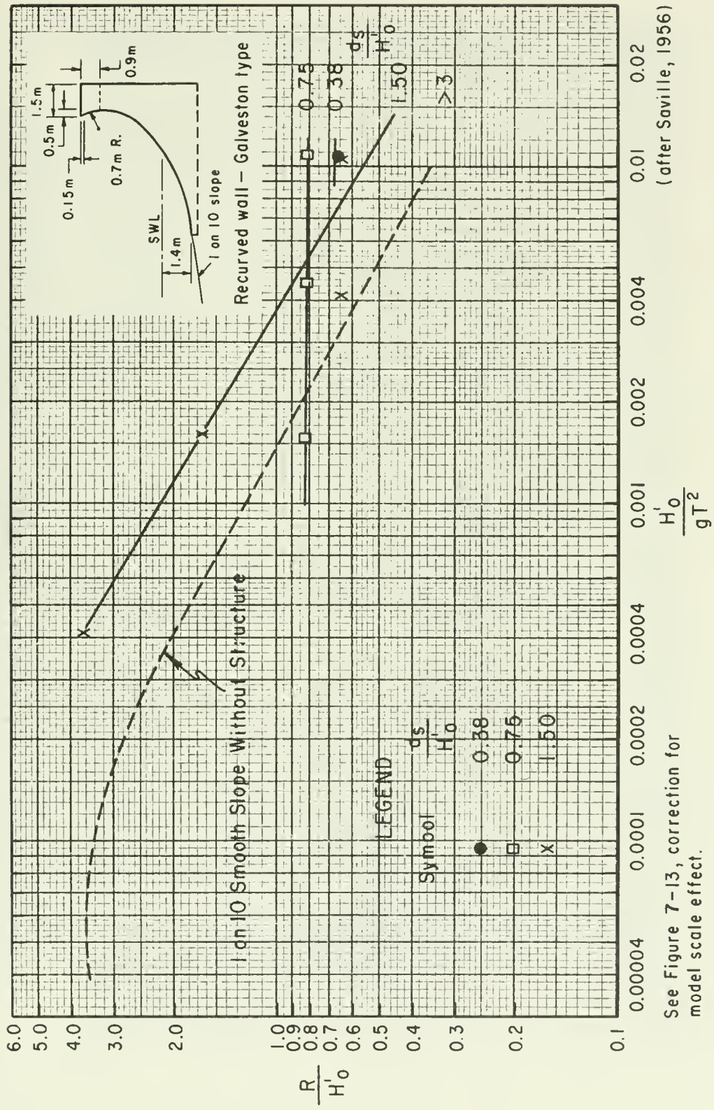
Figure 7-18. Wave runoff on recurved (Galveston-type) seawall versus H'_0/gT^2 .
