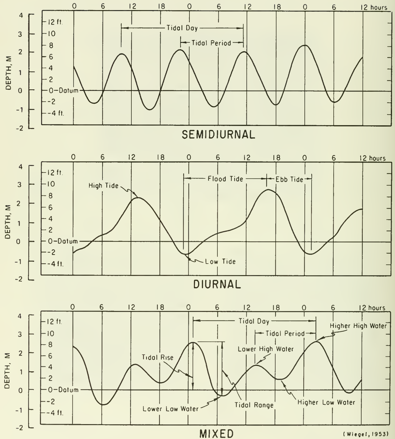
Figure A-10. Types of tides.
