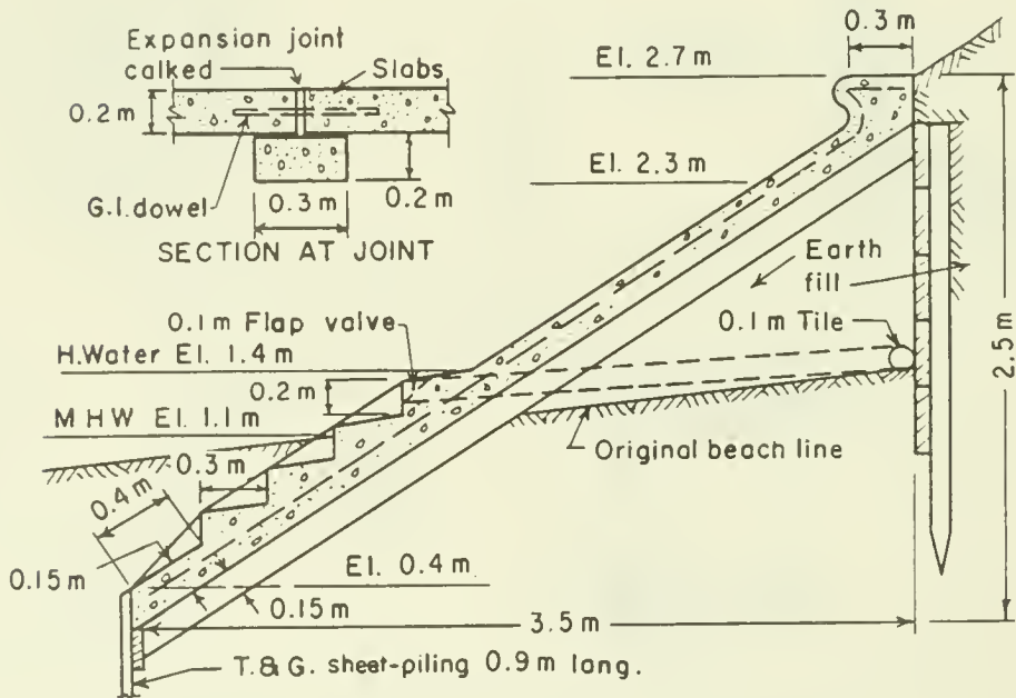
Figure 6-9. Concrete revetment.
