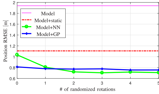
Fig. 10. The horizontal position error as dependent on to what extent the estimates utilize the rotational symmetry of the sensors.
