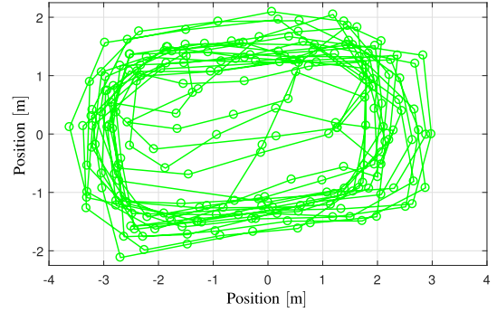
Fig. 9. Position estimates after neural network correction.
