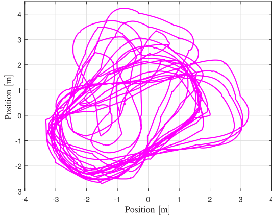
Fig. 6. Position estimates from foot-mounted inertial navigation system.
