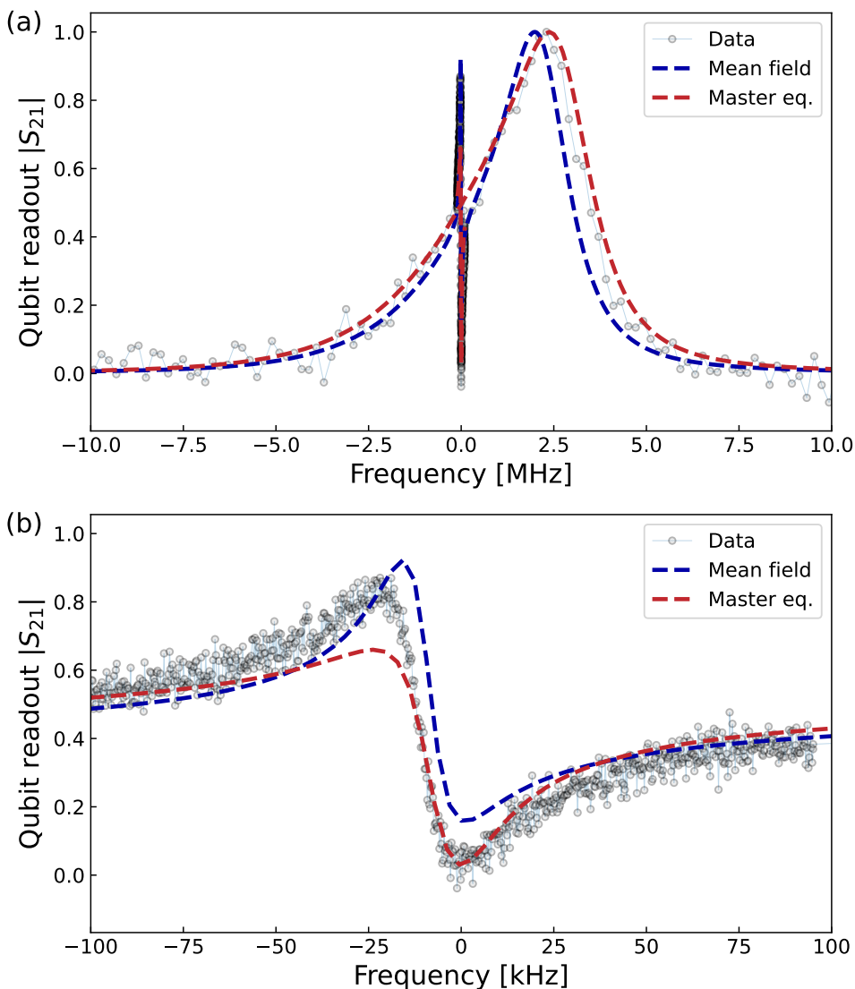
Figure 5.3: Two-tone qubit spectroscopy of AIT in qubit transition peak. Experimental two-tone data of qubit 01-transition coupled to a single HBAR mode at 6.064 GHz (grey dots). Both panels also show the qubit spectrum determined from mean-field (blue dashed line) and master equation simulations (red dashed line). (a) Full AIT of qubit with one coupled HBAR mode. (b) Zoom in of the HBAR mode.
