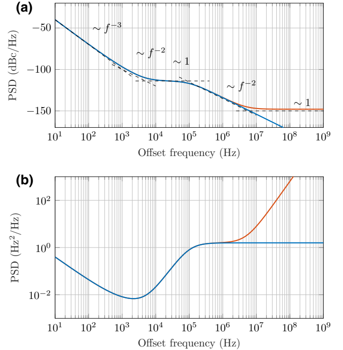
FIG. 3. A typical plot of (a) the phase noise and (b) the resulting frequency-noise PSD of a PLL-based frequency generator. The red line indicates the noise as measured by a phase-noise analyzer, whereas the blue line indicates the part of the noise that is actually phase noise. At high offset frequencies, where the lines diverge, wide-band additive noise shows up in the phase-noise plot, giving rise to a noise floor of around -150 dBc/Hz in this example.
