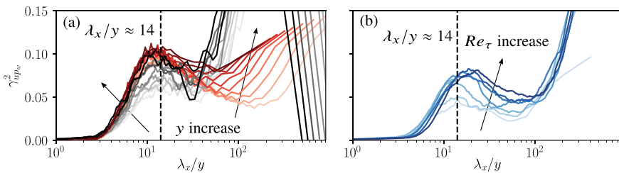
Fig. 3 a Coherence spectra of wall-pressure and streamwise velocity in the logarithmic region for DNS channel flow data (red, [12]) and experimental data (black, [11]) at Re_\tau \approx 2\,000 and for 10 logarithmically spaced locations in the range y^+ \in (80, 200) . b Coherence spectra of wall-pressure and velocity for data acquired in the CICLoPE facility
