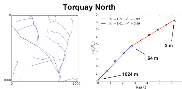
Figure 4. Sewer system (left) and computation of the corresponding fractal dimension, i.e. Eq. (1) in log–log plot (right), for the Torquay north study area. For the left figure, the axes correspond to metres (m).
