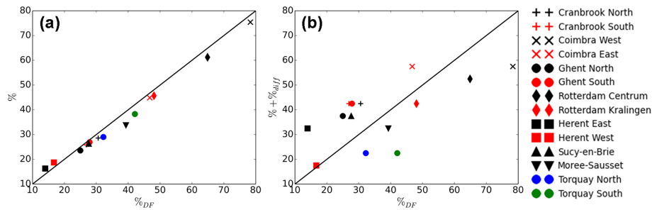
Figure 10. The percentages of distributed imperviousness (%) at the highest data resolution (a) and of the imperviousness of semi-distributed models (% + % diff ) (b) as a function of the percentages of imperviousness resulting from the fractal dimension estimates (% DF ). The black line indicates the first bisector.
