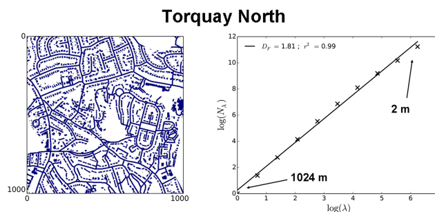
Figure 5. Impervious pixels at a 2 m resolution (left) and computation of the fractal dimension of the corresponding geometrical set, i.e. Eq. (1) in log–log plot, (right) for the Torquay north study area. For the left figure, the axes correspond to metres (m).
