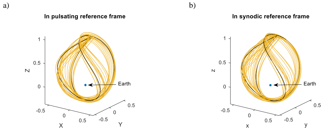
Figure 15 Effect of lunar eccentricity on the orbit of Figure 12b over one year with \phi_s = 0 . Black and yellow orbits are for e = 0 and e = 0.0549 , respectively. a) In pulsating reference frame. b) In synodic CR3BP reference frame.
