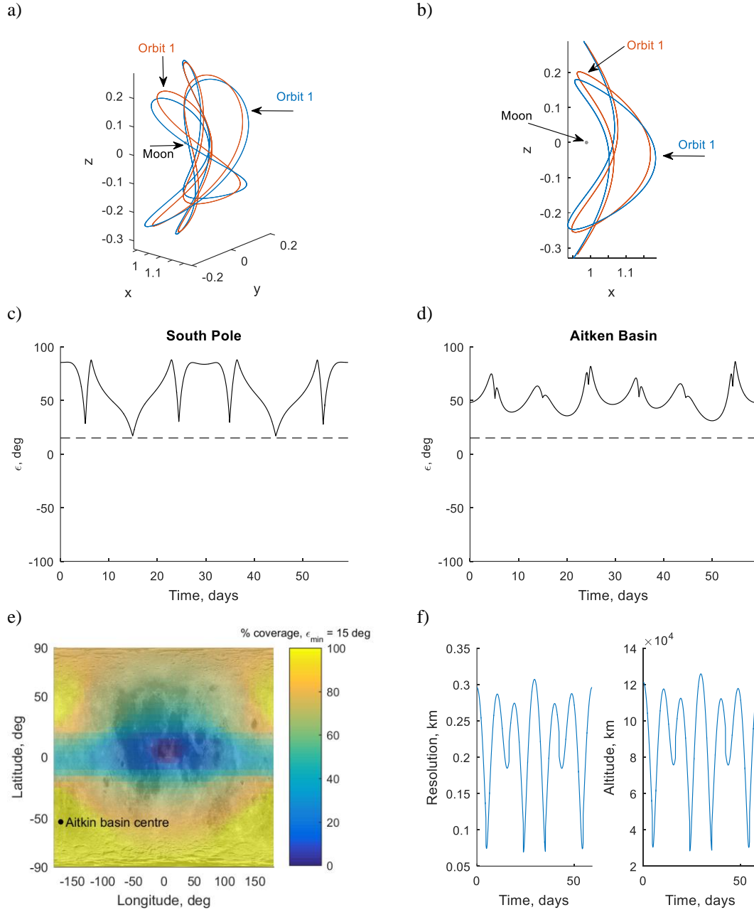
Figure 10 Constellation of solar sail L 2 vertical Lyapunov orbits. a,b) Constellation. c) Best elevation angle at lunar South Pole. d) Best elevation angle at center of Aitken Basin. e) Percentage temporal coverage for minimum elevation of 15 deg. f) Resolution and altitude (South Pole).
