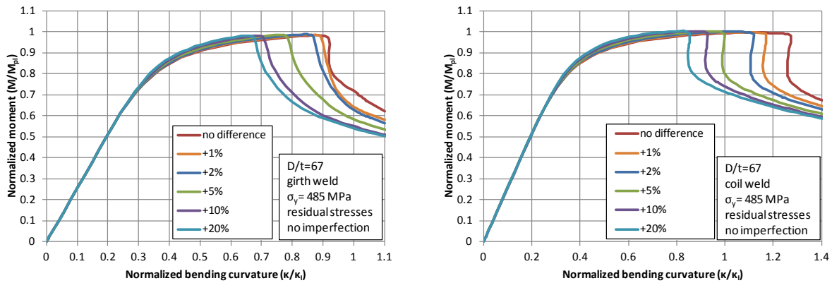
Fig. 14: Normalized moment-curvature diagrams of a 42-inch diameter tube ( D/t=67 , grade X70) for different yield stress values of connected tubular parts (girth welds and coil connection welds)
