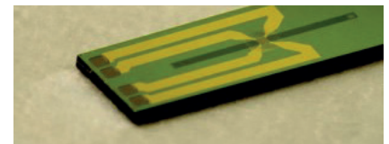
Figure 3. Nano reactor to study chemical reactions in-situ in a TEM. These are now commercialized together with the start-up DENSSolutions
