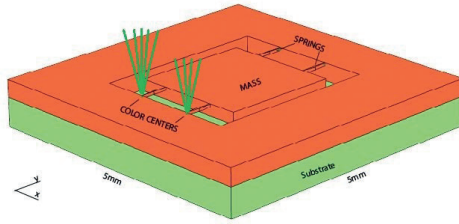
Figure 4. Quantum enhanced accelerometer design with diamond colour centres.
