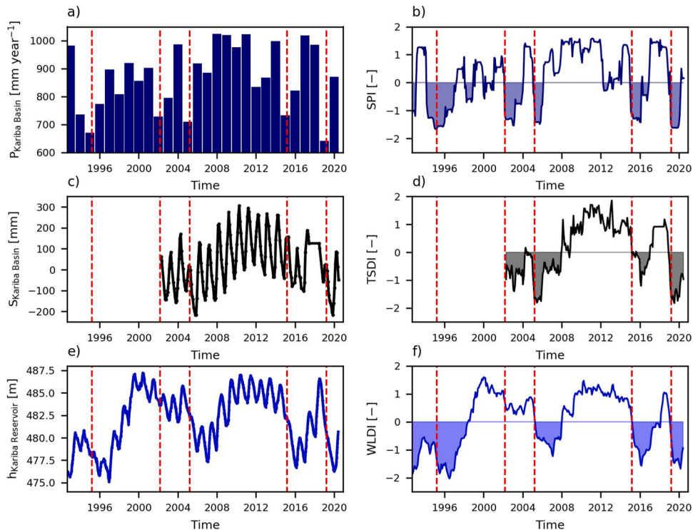
Fig. 2. a) Basin-averaged annual precipitation, b) monthly SPI (Standardized Precipitation Index), c) basin-averaged monthly total water storage anomalies, d) monthly TSDI (Total Storage Deficit Index), e) altimetry observations at Kariba Reservoir, and f) 10 – 35 day WLDI (Water-Level Deficit Index). The red dashed lines mark the dates 15 March 1995, 2002, 2005, 2015 and 2019 which were chosen visually to mark several extremely dry years.
