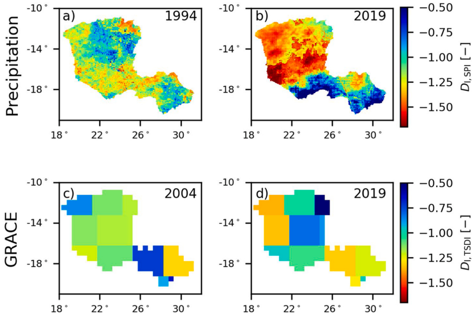
Fig. 5. Spatial variability of the drought intensity according to the precipitation (a – b) and according to the total water storage (c – d). The maps were temporally averaged considering the most severe drought according to precipitation (a) or GRACE (c), and the drought of 2019 (b and d).
