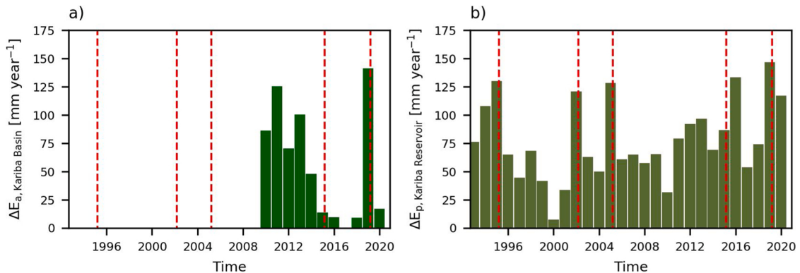
Fig. 3. Annual total a) actual evaporation for Kariba Basin; deviation from the minimum ( 888 \text{ mm year}^{-1} ) and b) potential evaporation for Kariba Reservoir; deviation from the minimum ( 1200 \text{ mm year}^{-1} ). The red dashed lines mark the dates 15 March 1995, 2002, 2005, 2015 and 2019, which were chosen visually based on Fig. 1 to mark several extremely dry years.
