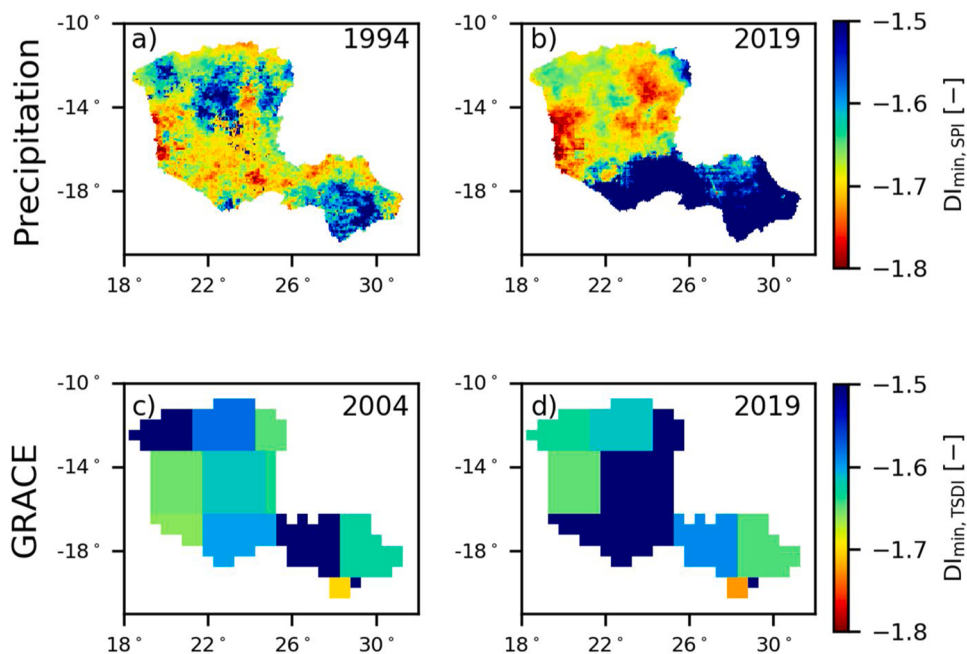
Fig. 4. Spatial variability of the minimum drought index according to the precipitation (a – b) and according to the total water storage (c – d) for the most severe drought according to precipitation (a) or GRACE (c), and the drought of 2019 (b and d).
