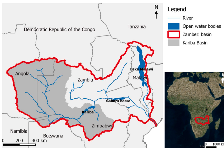
Fig. 1. Map of the Zambezi River Basin and the basin area upstream of the Kariba Reservoir now called “Kariba Basin”.
