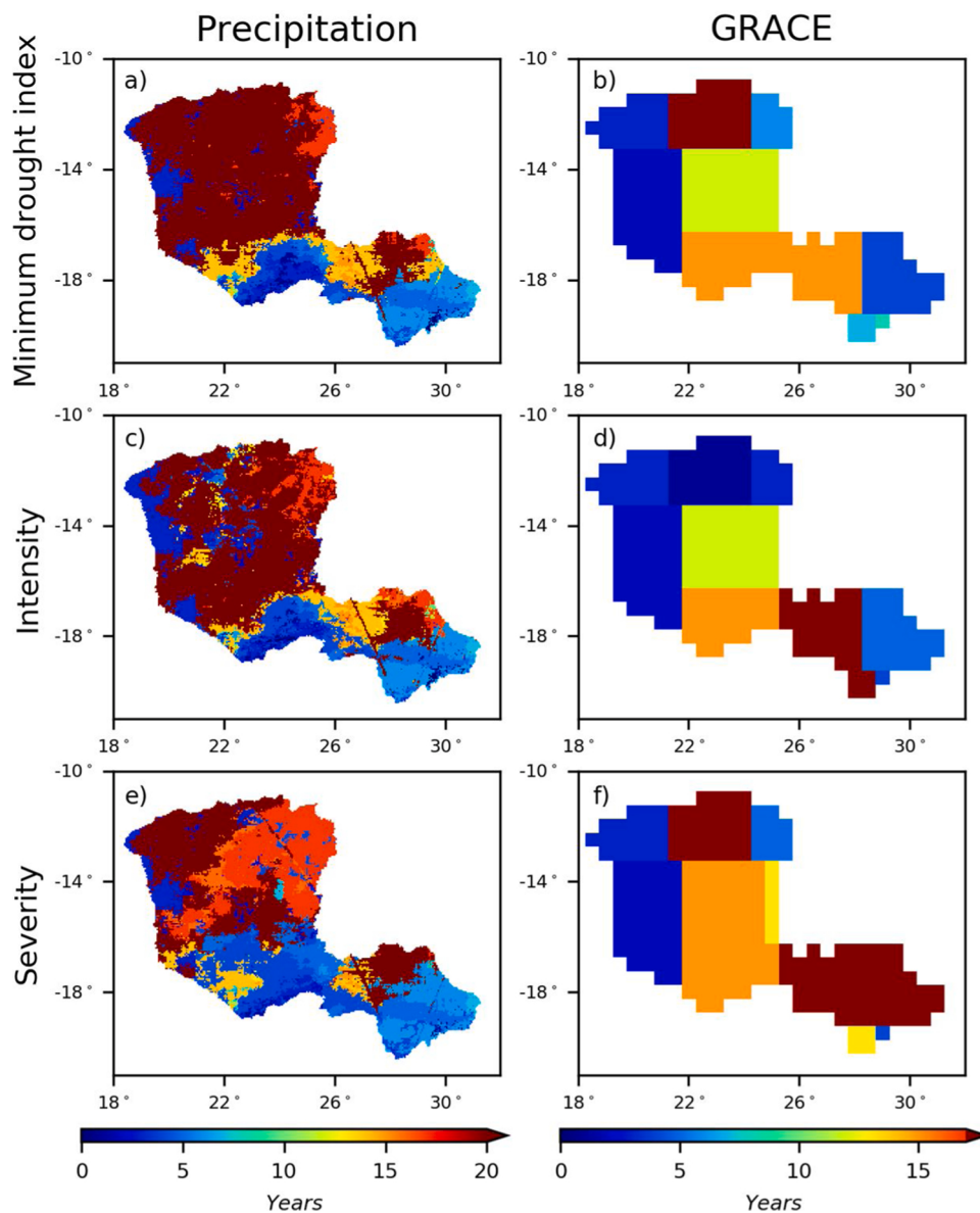
Fig. 7. Spatial variability of the number of years between the drought of 2019 and the most recent drought before 2019 with more extreme values based on the minimum deficit index (a and b), drought intensity (c and d) and drought severity (e and f) according to precipitation (a, c and e) or GRACE data (b, d and f). Grid cells where the drought of 2019 was the most severe as observed with satellite data are colored dark red.
