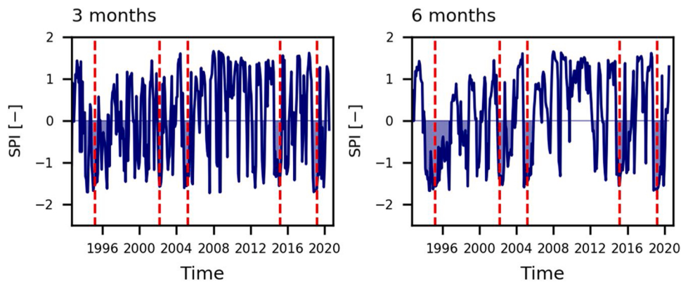
Fig. 8. Basin-averaged SPI using 3 or 6 preceding months.
