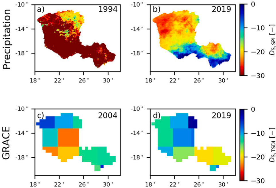
Fig. 6. Spatial variability of the drought severity according to the precipitation (a – b) and according to the total water storage (c – d). The maps were temporally averaged considering the most severe drought according to precipitation (a) or GRACE (c), and the drought of 2019 (b and d).
