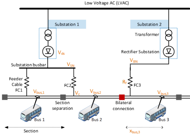
Fig. 1. Trolleygrid and its components.
