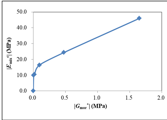
Figure 8. Relationship between |E_{mix}^c| and |G_{mor}^*| .
