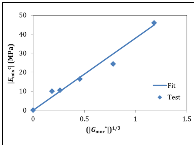
Figure 9. Relationship between |E_{mix}^c| and |G_{mor}^*|^{1/3} .
