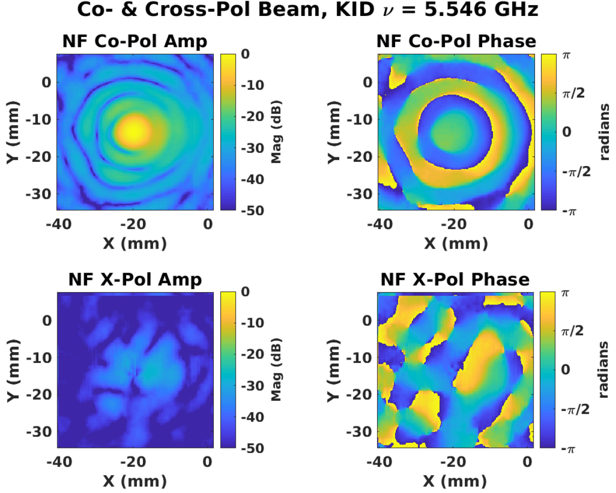
Fig. 3. Near-field co-polarization (upper two panels) and cross-polarization (bottom two panels) beam maps for the same representative pixel as shown in Fig. 2. The left two panels show the amplitude, scaled to the peak of the co-polarization map, and the right two panels show the phase structure. The image has been cropped to a square 8 \times the beam width, centered on the amplitude peak in the co-polarized map to cut out the wide-field noise.
