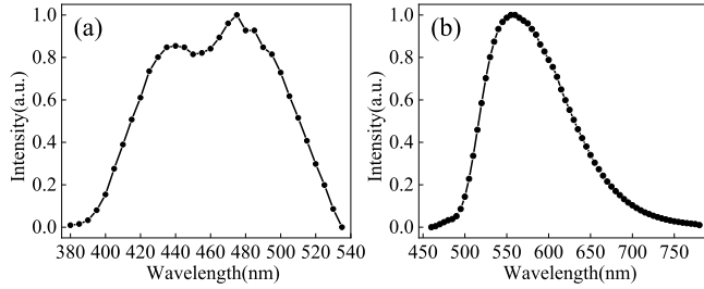
Fig. 4. (a) The excitation spectrum and (b) The emission spectrum of YAG: \text{Ce}^{3+} phosphor used in this study.
