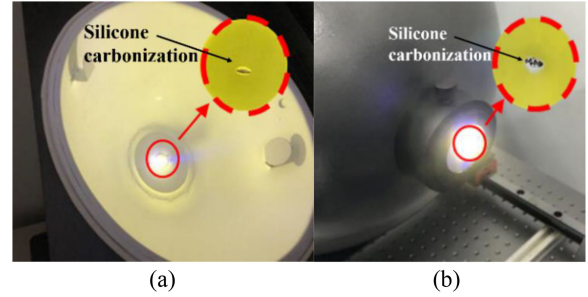
Fig. 6. The carbonization of YAG: \text{Ce}^{3+} phosphor/silicone composites excited by 0.68 W blue laser: (a) R-mode; (b) T-mode.
