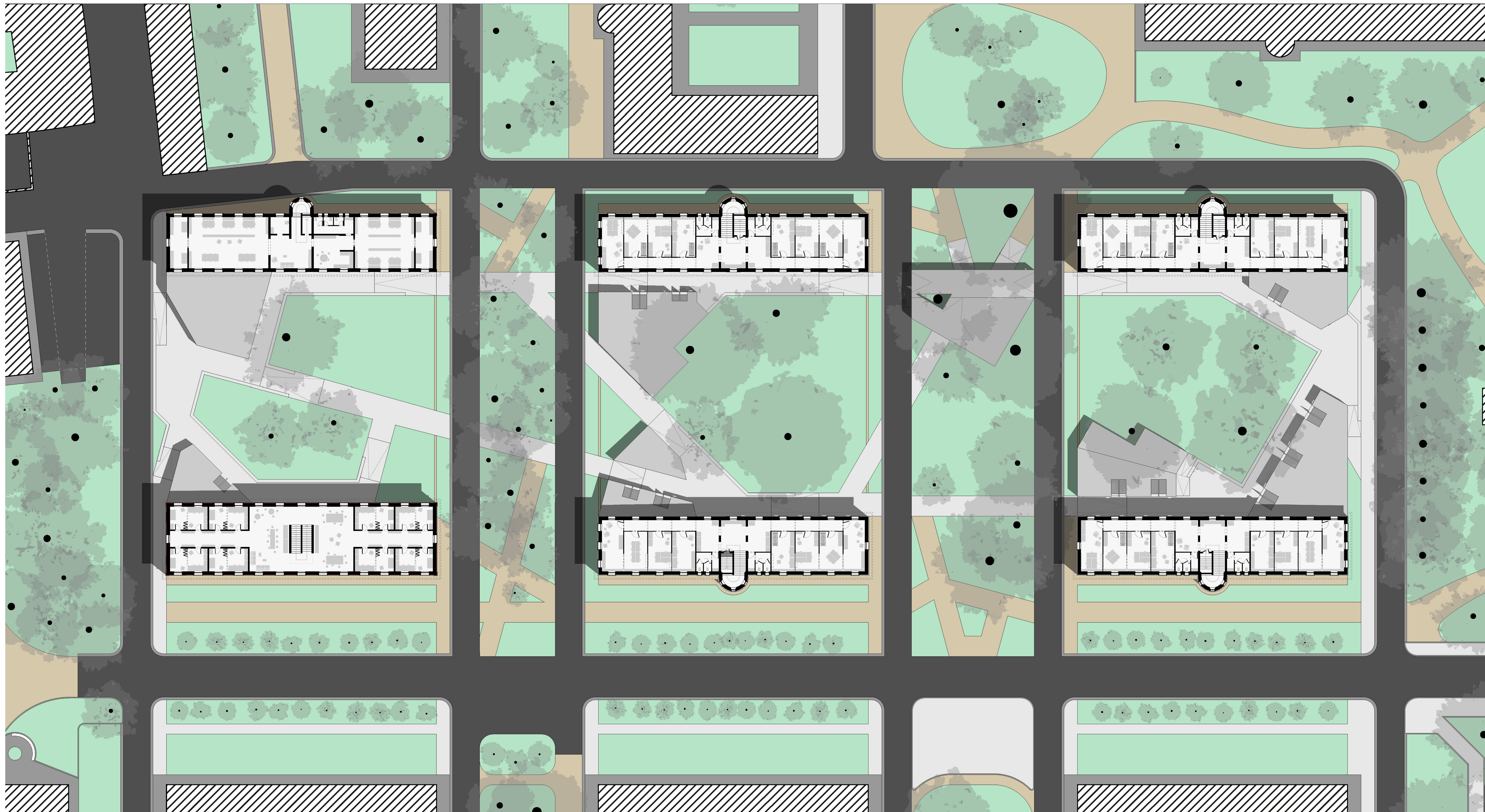
- First floor of the intervention - Scale 1:200
