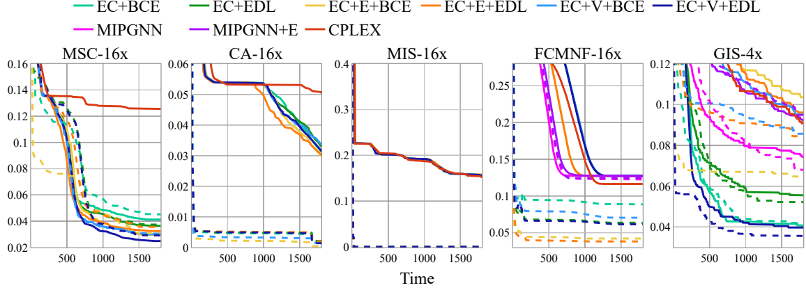
Figure 7: Average Primal Gap Curves for the Largest Scale Transfer Datasets. NS and UPR+NS curves are denoted by solid and dashed lines, respectively. To present the primal gap value averaged across all instances per second by a CO pipeline, primal gap values are linearly interpolated through the time interval [1, 1800] .
