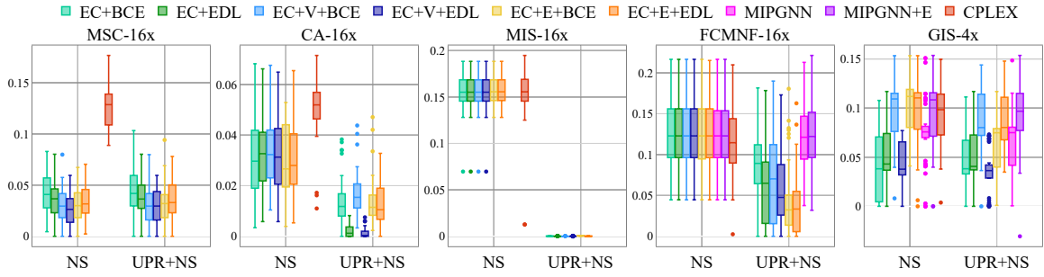
Figure 4: Primal Gap Distributions for the Largest Scale Transfer Datasets
