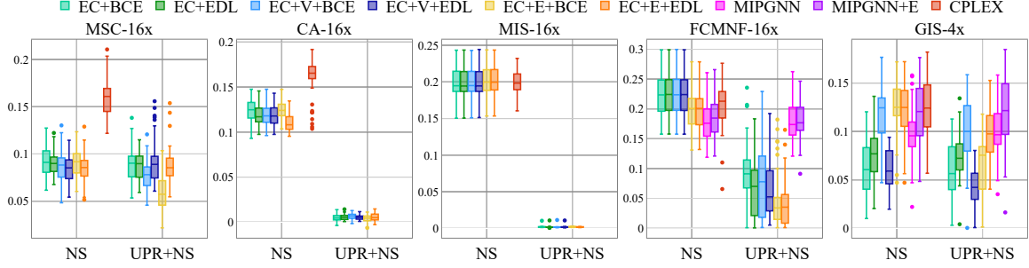
Figure 5: Primal Integral Distributions for the Largest Scale Transfer Datasets
