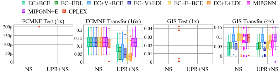
(b) Primal Gap Distributions for FCMNF and GIS Datasets
