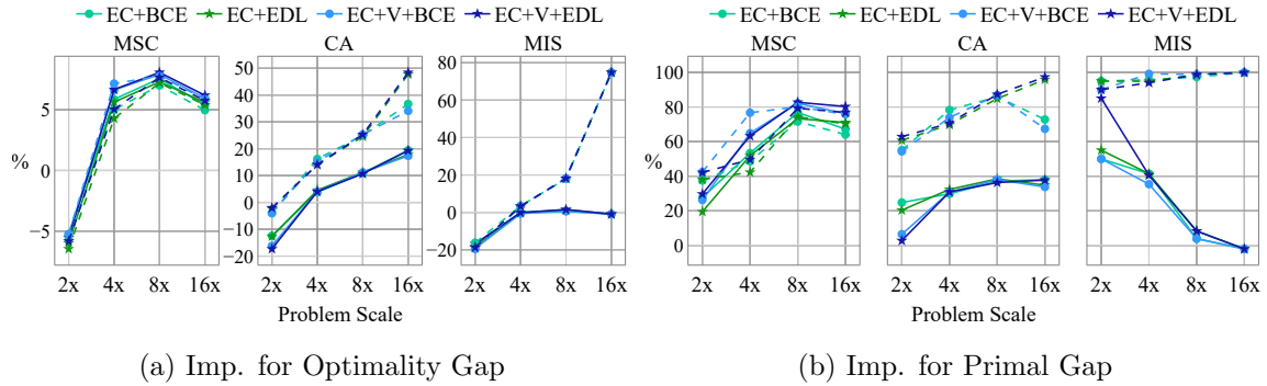
Figure 8: Average Improvement Rates (Imp.) by the Model Configurations for the Transfer Datasets of MSC, CA, and MIS Problems (NS and UPR+NS results are denoted by solid and dashed lines, respectively.)
