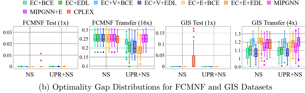
Figure 13: Optimality Gap Distributions for All Datasets
