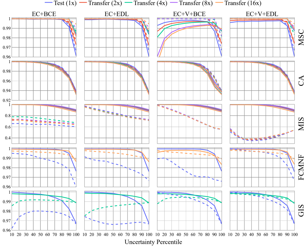
Figure 12: Average Accuracy of the Predicted Decision Values by the Models with (solid curves) and without (dashed curves) the Proposed Normalization Techniques in Each Uncertainty Percentile for All Datasets
