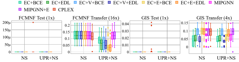
(b) Primal Integral Distributions for FCMNF and GIS Datasets
