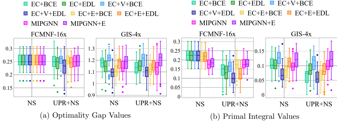
Figure 11: Optimality Gap and Primal Integral Distributions by the CO Pipelines Using the Models with 4-layered GNN and mean aggregation, and MIP-GNN models for FCMNF-16x and GIS-4x Transfer Datasets
