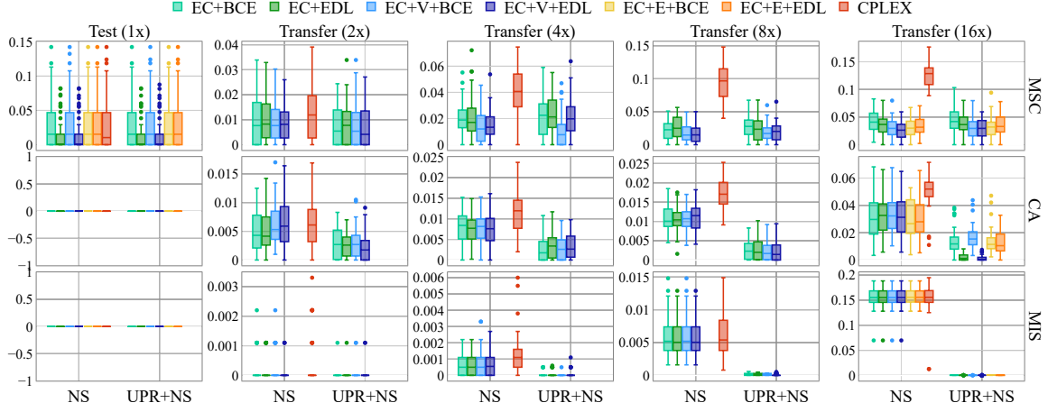
(a) Primal Gap Distributions for MSC, CA, and MIS Datasets
