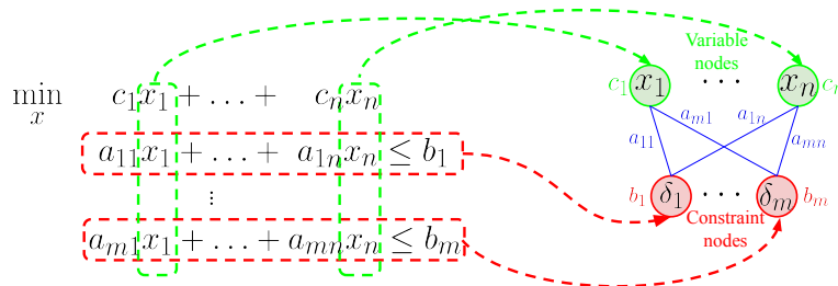
Figure 1: MIP Representation as a Bipartite Graph. Image credit to (Nair et al., 2020).
