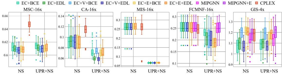
Figure 3: Optimality Gap Distributions for the Largest Scale Transfer Datasets
