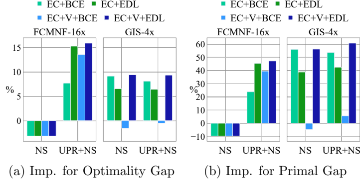
Figure 9: Average Improvement Rates (Imp.) by the Model Configurations for the FCMNF-16x and GIS-4x Datasets
