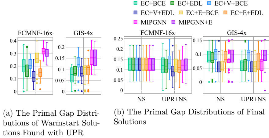
Figure 10: Primal Gap Distributions of Warmstart (10a) and Final (10b) Solutions by the CO Pipelines Using 4-layered GNNs and mean aggregation for FCMNF-16x and GIS-4x Transfer Datasets
