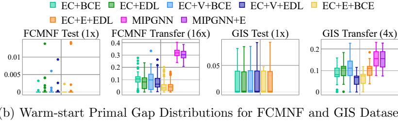
Figure 16: Primal Gap Distributions of Warm-start Solutions through UPR Algorithm for All Datasets
