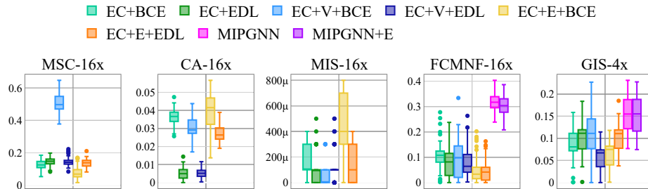
Figure 6: Primal Gap Distributions of the Warm-start Solutions Found with UPR for the Largest Scale Transfer Datasets
