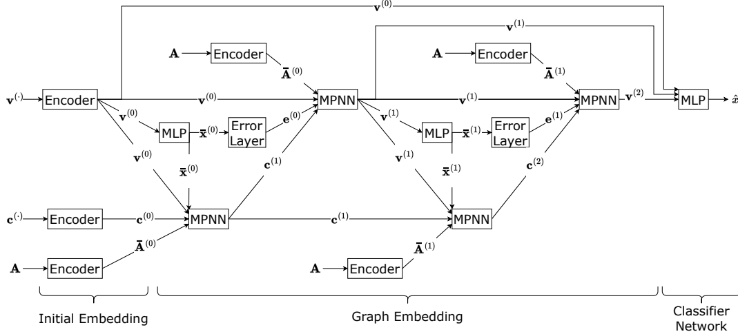
Figure 2: MIP-GNN Architecture with Two-Layer Graph Embedding
