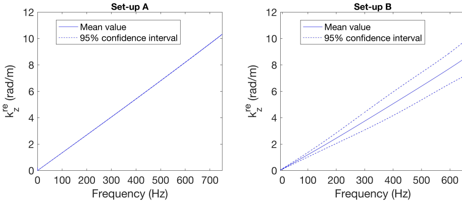
Figure 5.6: The real part of the axial wavenumber k_z^{re} as a function of frequency for Set-up A (left) and Set-up B (right). k_z here represents the wavenumber of the axisymmetric water-borne wave. The results were obtained by processing the raw signals according to the procedure described in Figure 5.2.
