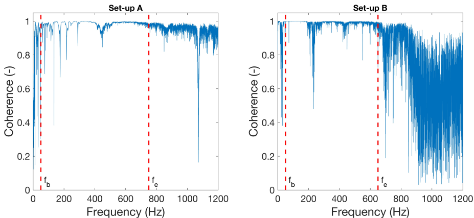
Figure 5.4: The coherence as a function of frequency between the hammer and the single hydrophone signal in Set-up A (left) and between the two hydrophone signals Set-up B (right). In each case, the coherence is estimated from Eq. 5.1. The red dashed lines show the frequencies f_b and f_e used in the Butterworth frequency filter.
