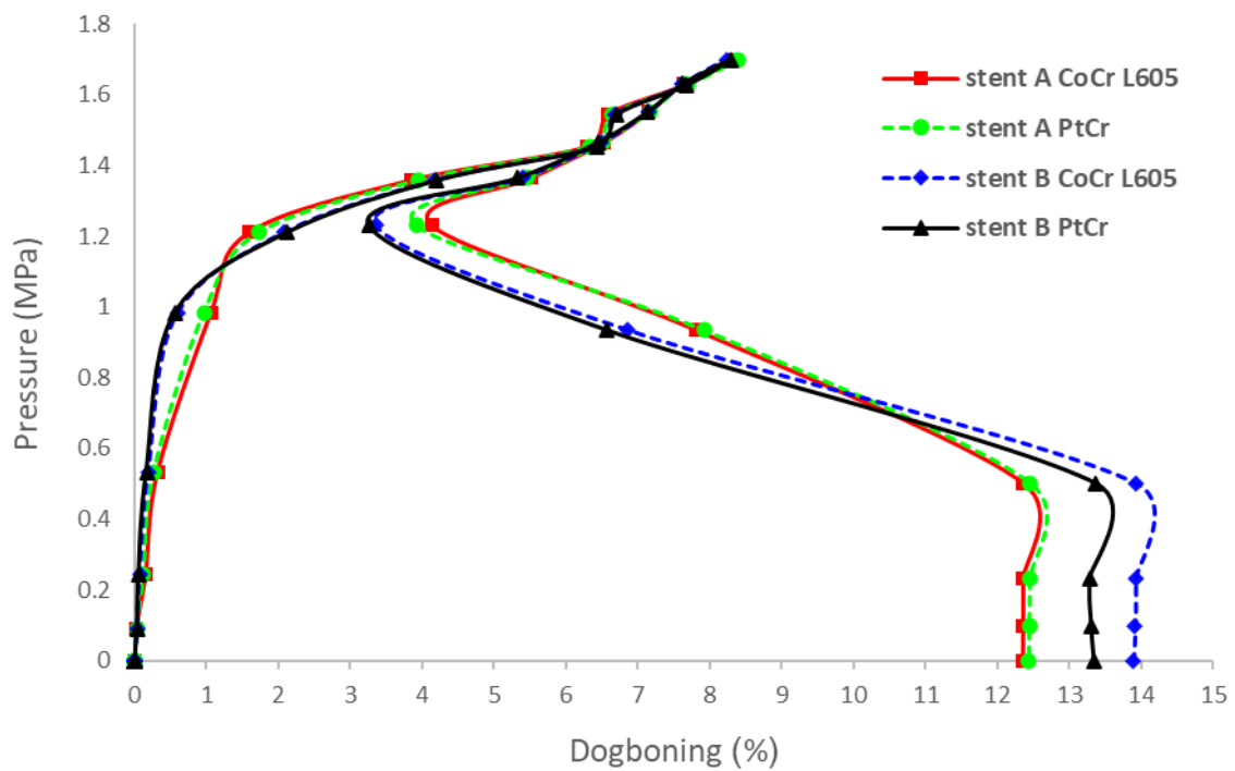
Fig. 21- Diagram of dogboning change in terms of pressure (During the loading and unloading steps) for stent A CoCr L605, stent A PtCr, stent B CoCr L605 and stent B PtCr.
