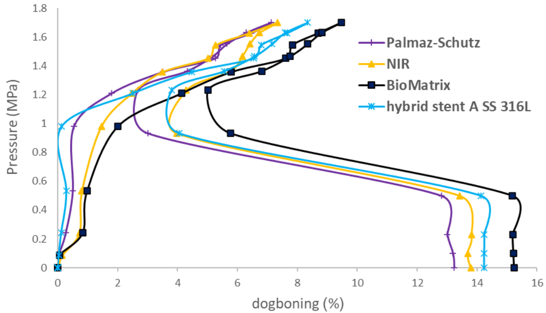
Fig. 12- Diagram showing the variation of dogboning with balloon pressure for Palmaz-Schatz, NIR, BioMatrix and hybrid stent A Ss 316L.
