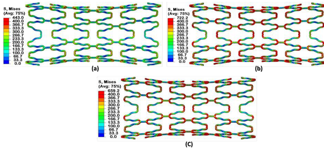
Fig. 14- The von Mises stress distribution for (a) stent A SS 316L, (b) stent A CoCr L605 and (c) stent A PtCr at the end of the unloading step.
