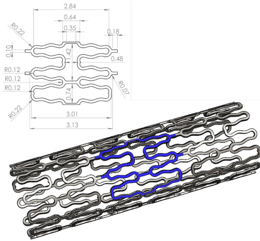
Fig. 1- New hybrid stent and geometric dimensions of each cell unit.
