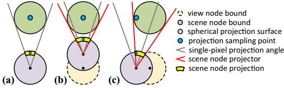
Figure 7: Discrepancies of scene-node projections for vertical (b) and horizontal (c) displacement of a child view against the projection for the centre of the view node (a).
