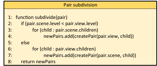
Figure 8: Pseudocode for pair subdivision for octree structures.
