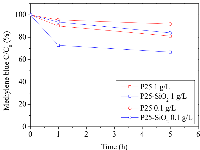
Figure 6. Adsorption of methylene blue along time for different concentrations of P25 and P25- \text{SiO}_2 .
