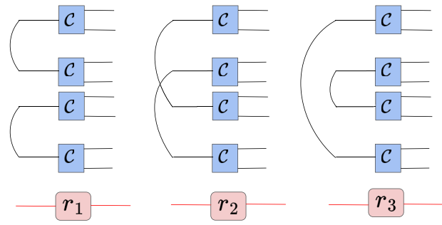
Figure 3. The different ways of partitioning a quantum system of N=4 size into d=2 groups. The three distinct configurations are superposed in the input state \psi and can be accessed by the state of the reference r .
