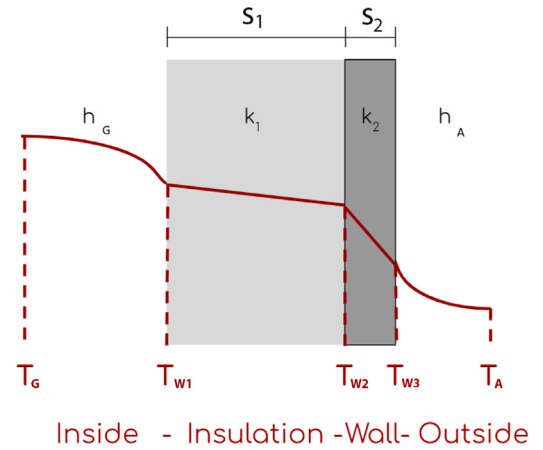
Fig. 4. Schematic of the heat flow through the autoclave wall. Temperature ranges from T_G (inside the autoclave), to T_A (outside the autoclave). It shows the thickness and thermal conductivity of the insulator (W1) and the steel wall (W2), and the convective heat transfer coefficients of the nitrogen gas (G) and the outside air (A).
