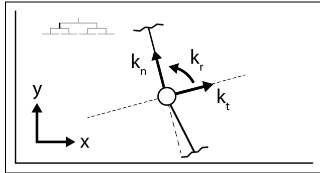
Figure 7. Normal-, shear-, and rotational stiffness acting on each individual joint in the whiffletree.
