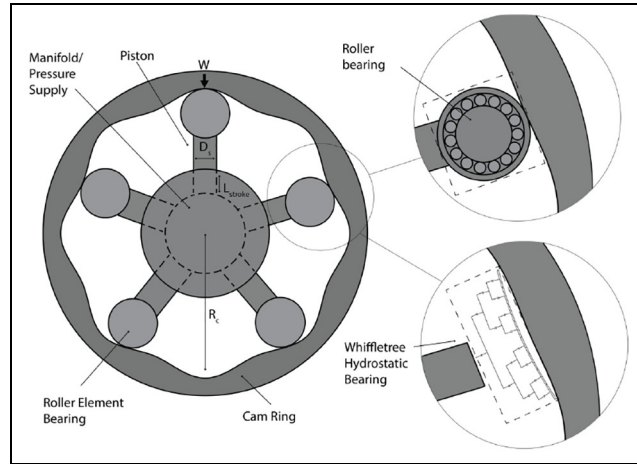
Figure 9. Schematic overview of the radial pump used in the case study where the conventional roller bearing and the newly obtained whiffletree supported hydrostatic bearing are shown.
