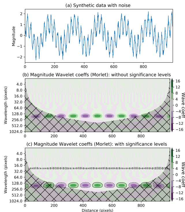
Figure A3. Example of why a significance test is needed. Panel (a) is a 1D synthetic, noisy signal made of two waves of different wavelengths. Panels (b) and (c) present the 1D wavelet transformation of (a) with a 1D Morlet wavelet. In (b), the result is only visualised, while in (c) the significance test is also visualised. In both, the hatched area contains edge effects and is delimited by a 1D cone of influence. The contouring in (c) shows domains that are within the 95 % confidence level of not being white noise. The contours highlight values that are both positively and negatively larger than the white noise model. The takeaway message is that the significance test is needed to accurately identify regions of “real anomaly”.
