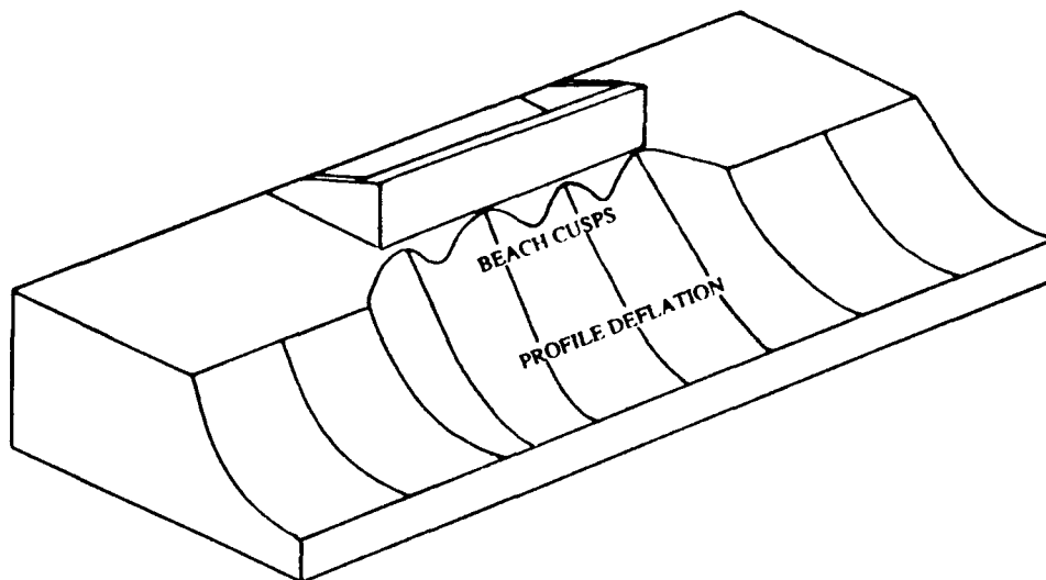
Figure 2. Types of beach response observed by Griggs and Tait before berm retreats past seawall
