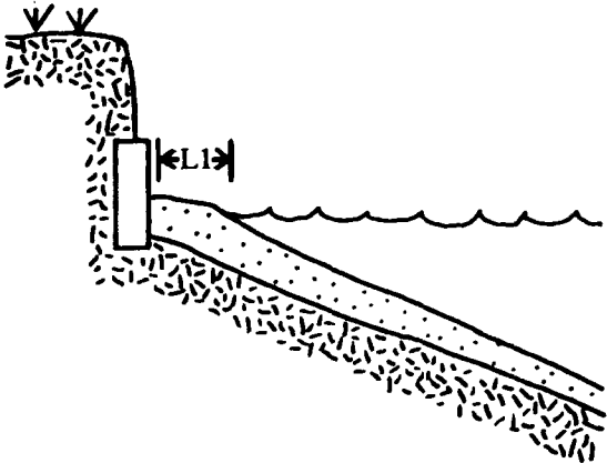
Figure 22. Long term effects of a seawall on a retreating shoreline
