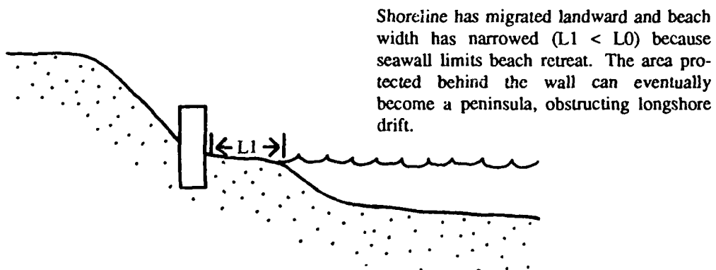
Figure 21. Long term effects of a seawall on a retreating shoreline
