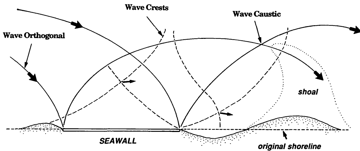
Figure 18. Short-crested wave system generated by obliquely reflected waves summing with incident waves. Areas of scour are produced in the vicinity of the wall and deposition occurs further downcoast. (From Silvester 1977)
