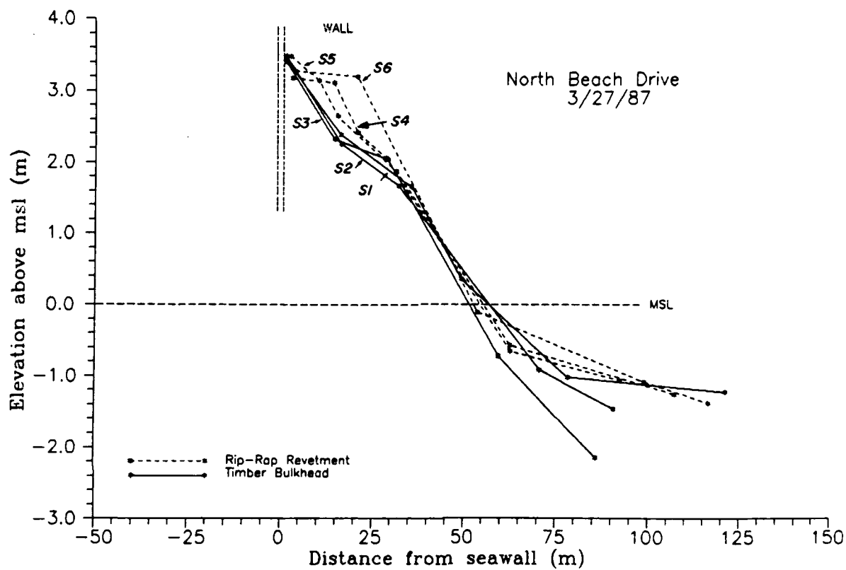
Figure 20. Beach profiles at North Beach Drive. Note persistence of wide berm in front of permeable revetment (dashed lines) in contrast to absence of berm in front of impermeable bulkhead (solid lines). (From Griggs and Tait 1988)
