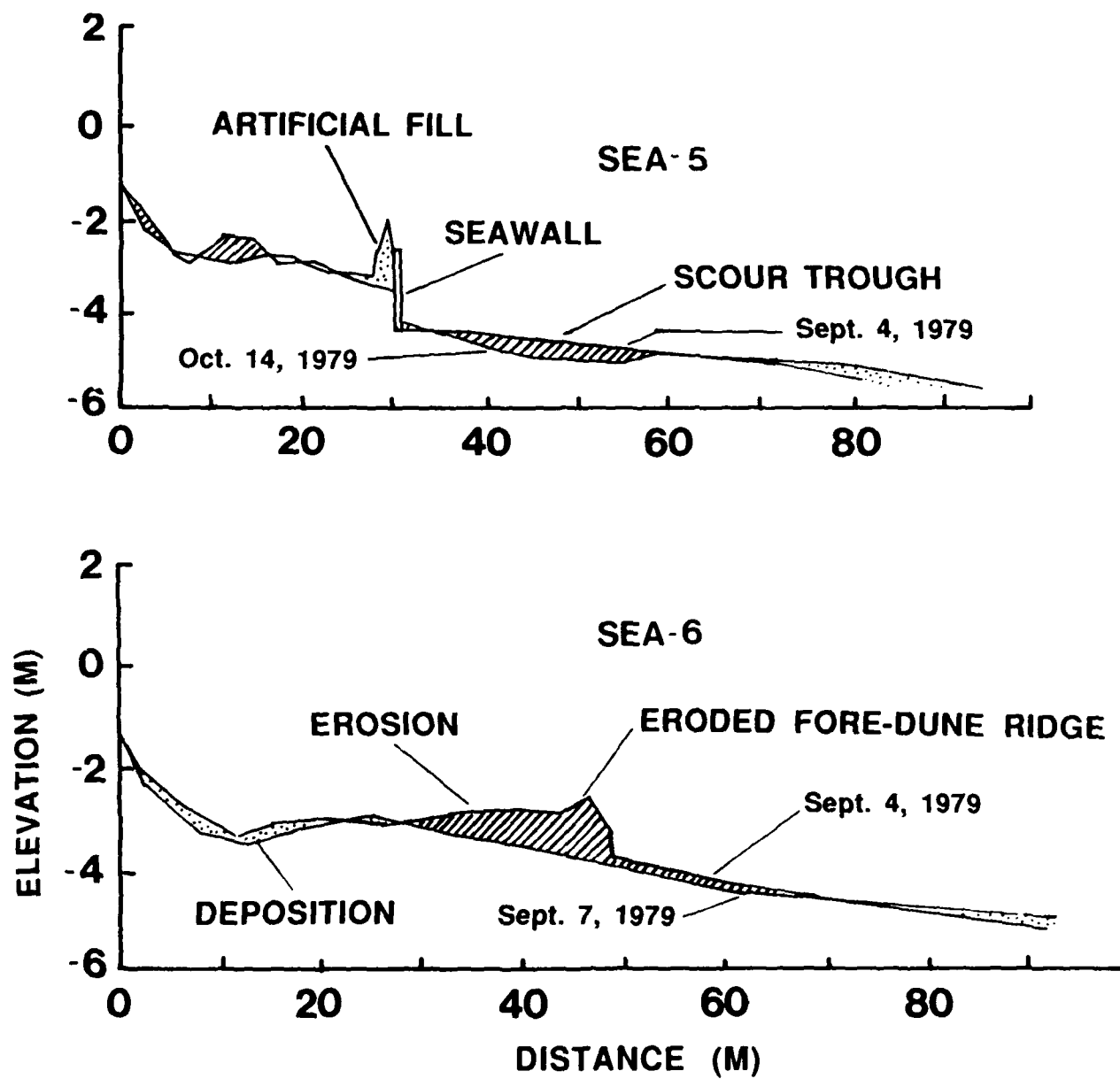
Figure 5. Pre- and post-storm profiles, Seabrook Island (Sexton and Moslow 1981)
