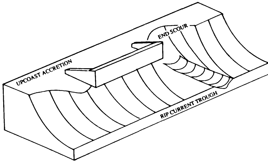
Figure 3. Types of beach response observed by Griggs and Tait after berm retreats past seawall
