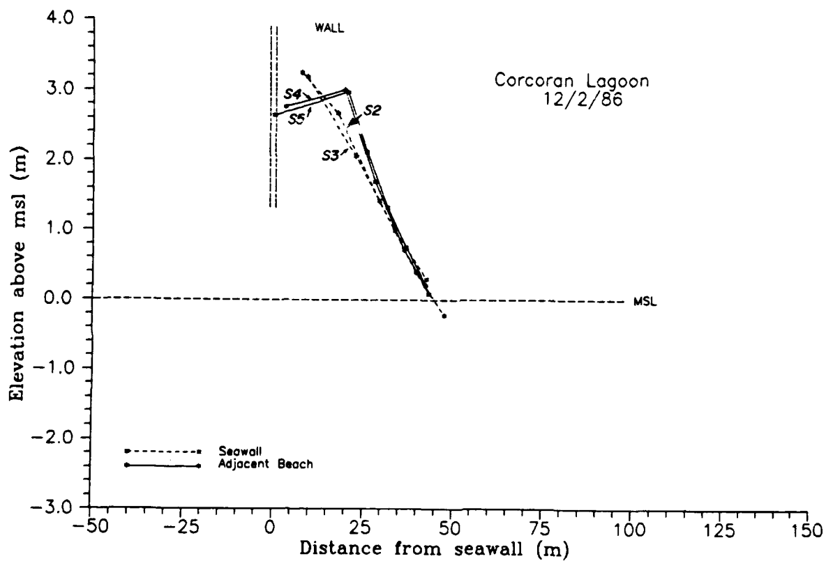
Figure 10. Beach profiles at Corcoran Lagoon, Monterey Bay, showing deflation of summer berm in front of seawall (dashed lines) and persistence of berm on adjacent natural beach (solid lines). (From Griggs and Tait 1988)
