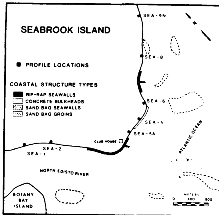
Figure 4. Location map of profile stations and structures in Sexton and Moslow study of the effects of Hurricane David on Seabrook Island. Note location of profiles Sea-5 and Sea-6 discussed in text. (From Sexton and Moslow 1981)
