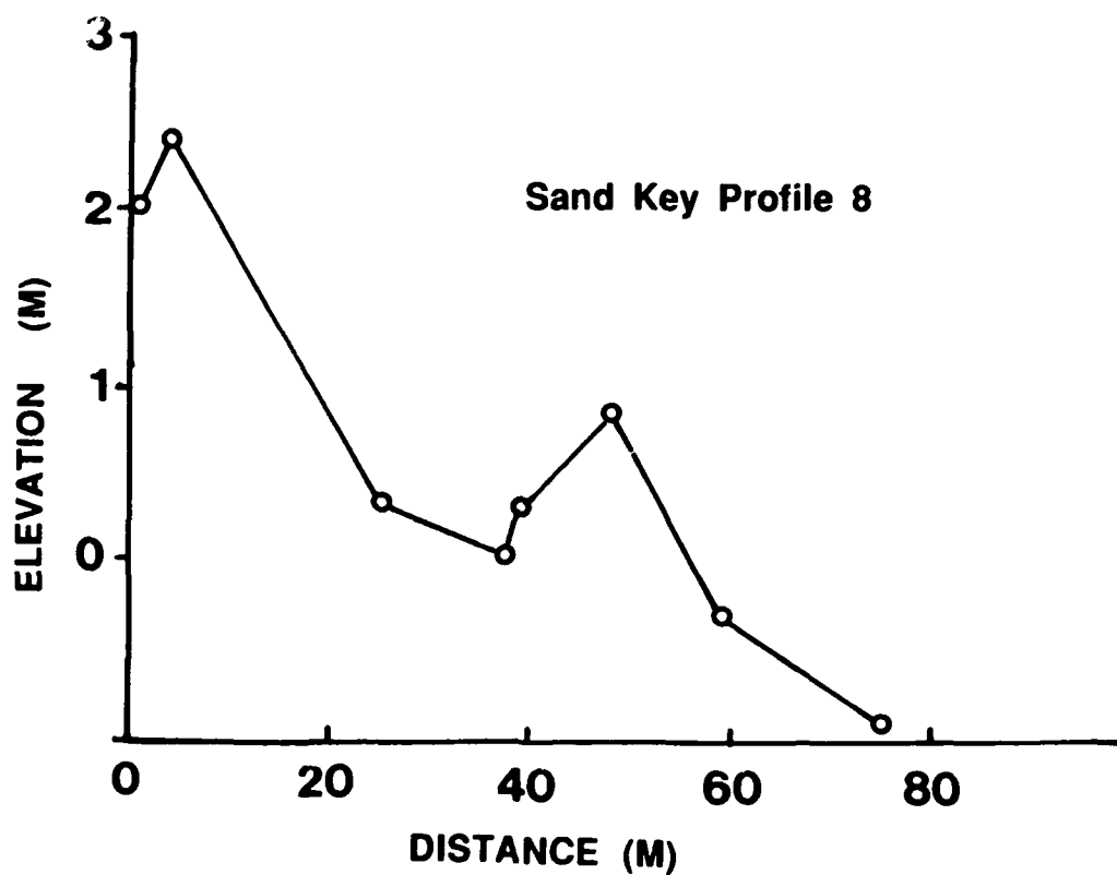
Figure 7. Post-storm profiles at Sand Key, Florida (Davis and Andronaco 1987)
