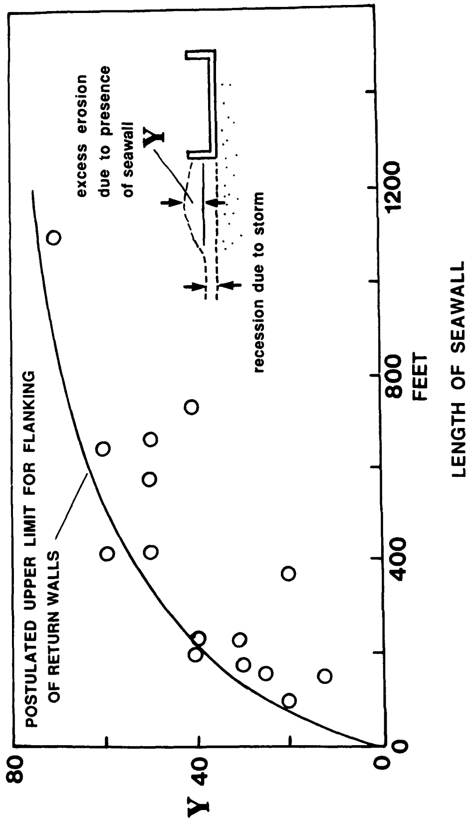
Figure 15. Graph of seawall length versus end scour (Walton and Sensabaugh 1979) (To convert feet to meters, multiply by )
