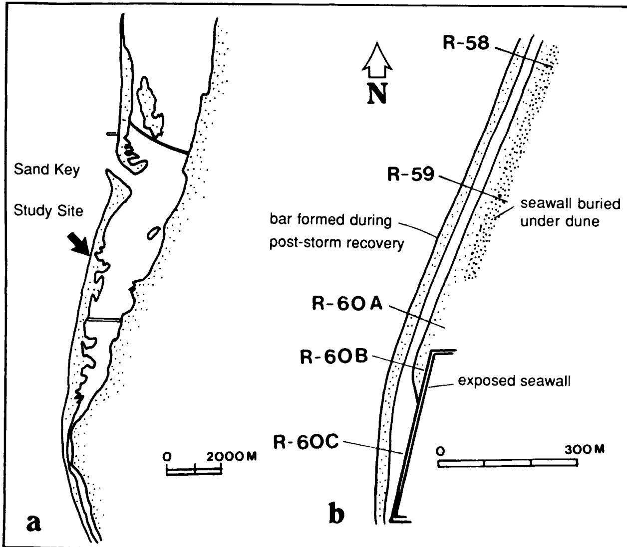
Figure 8. Site map for Sand Key, Florida study (Kriebel 1987)
