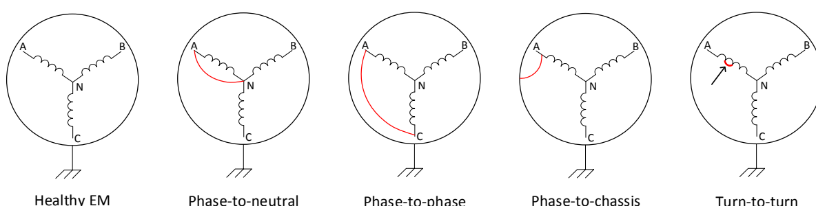
Figure 8. Identified short-circuit possibilities within EM
