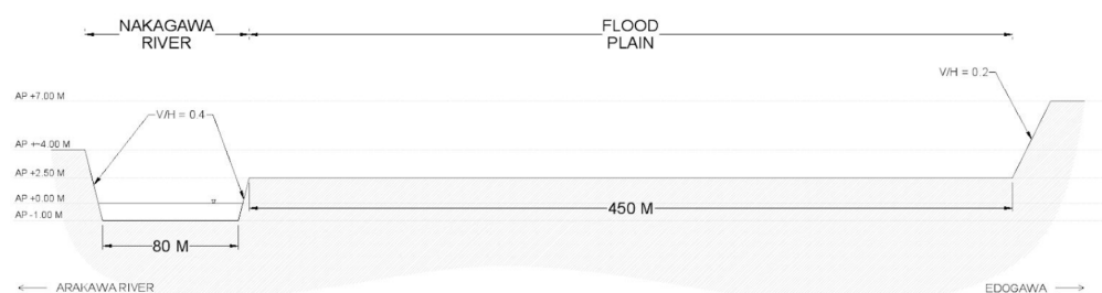
Figure 10. Simplified cross-section of Nakagawa River (source: Google Earth and Arakawa Karyu River Office [14]).
