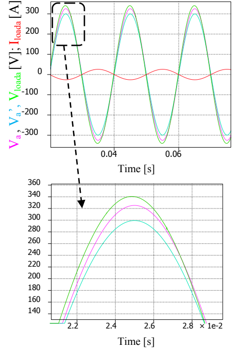
Fig. 11.3 - Steady state phase voltages [V] at input V_x and output V_x' of OLTC as a function of time [s]. An active DG is connected at the load end of the LV OLTC system which is set to -8% compensation
