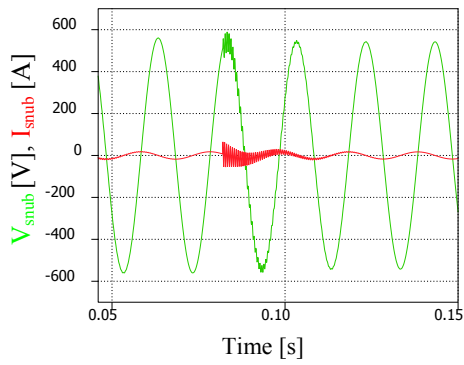
Fig. 11.7 - Transient voltage V_{\text{snub}} [V] and current I_{\text{snub}} [A] of snubber capacitor during 4-step commutation from BS2 to BS1 in MV OLTC, depicting the LC oscillation between leakage impedance and snubber capacitance of 100 \mu\text{F} for the scenario depicted in Fig. 11.4
