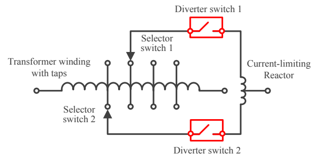
Fig. 4. Diverter switch type voltage regulator using no-load ‘selector’ switch [6]. Only two ‘diverter’ switches are required regardless of number of taps
