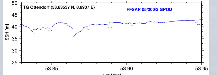
Figure 3. Water heights from FF-SAR at Ottendorf (red track in Fig. 1).
