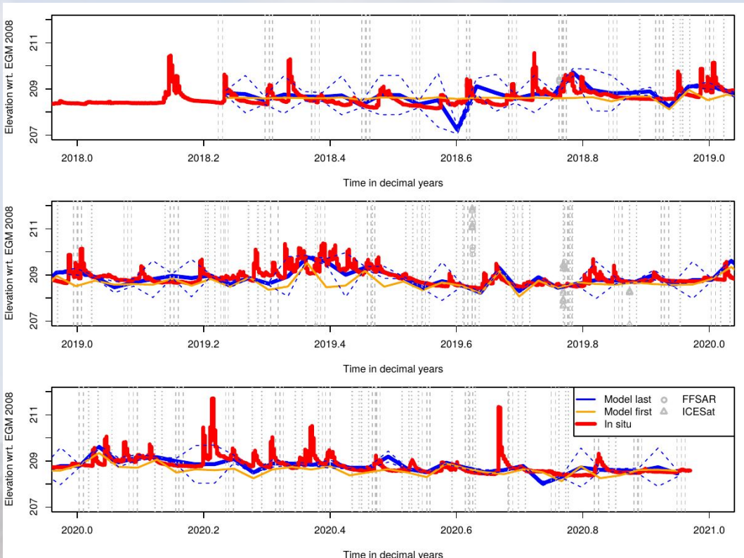
Figure 2: The reconstructed water level time series (blue) compared to the gauge water levels (red). The gray lines indicates the times where data is available
