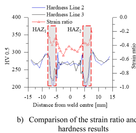
Fig. 5. Identification of the HAZ boundary.
