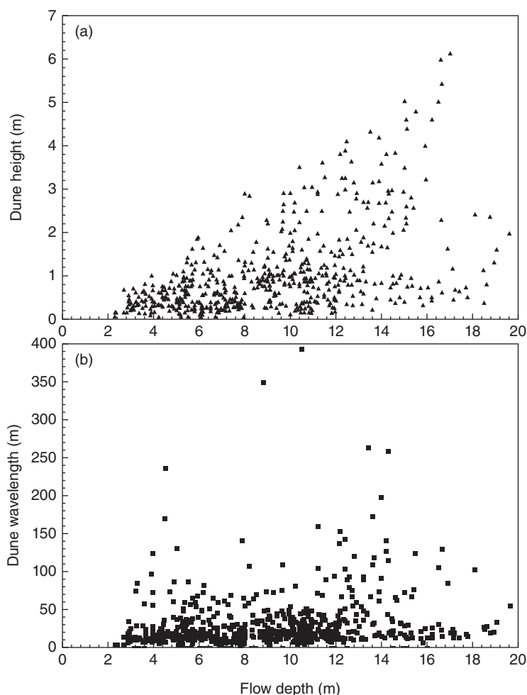
Figure 20.14 Plots of (a) dune height and (b) dune wavelength as a function of flow depth. Source: Based on FAP24 (1996g).
