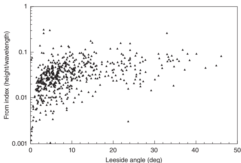
Figure 20.12 Form index of dunes in the Jamuna River as a function of leeside angle. Source: From Roden 1998.
