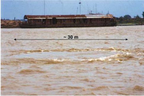
Figure 20.17 Macroturbulence erupting on the water surface of the Jamuna River near Bahadurabad: this locality was above a field of 3–4 m high dunes at the time of survey (Best 2005). Flow left to right, and flow depth ~15 m. For video of such turbulence, see https://www.youtube.com/watch?v=RMfaVJliK8 .
