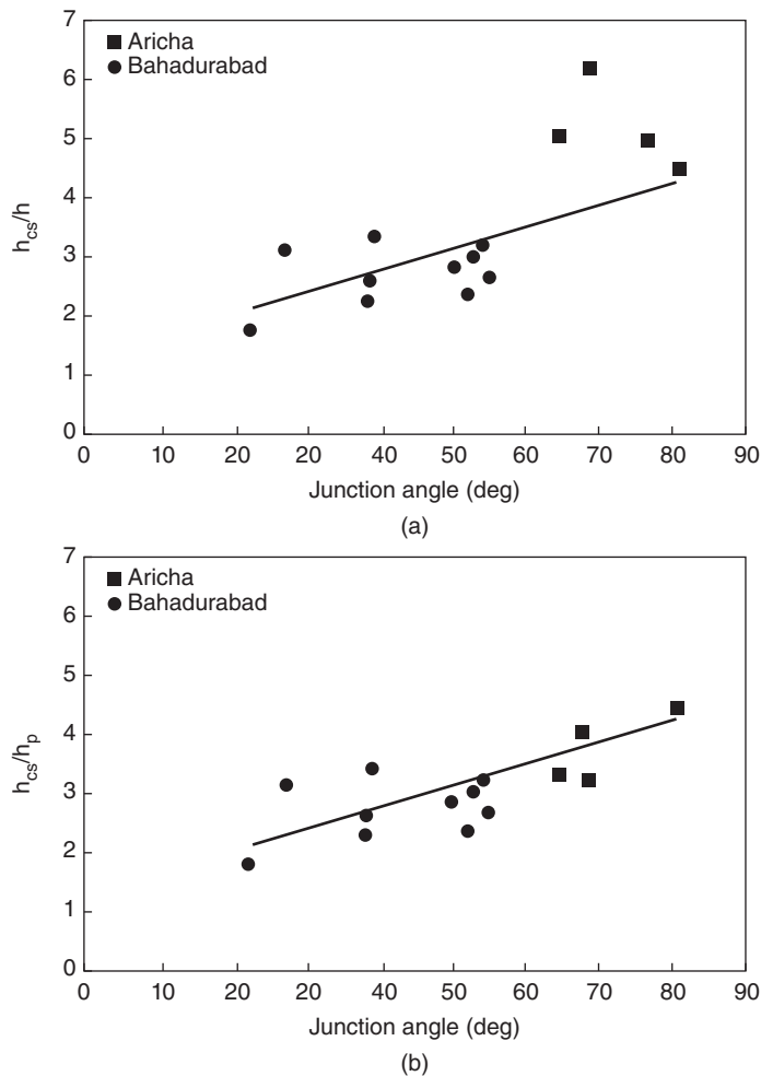
Figure 20.21 Confluence scour depth as a function of junction angle for data collected on the Jamuna River at Bahadurabad and Aricha: (a) with scour depth, h_{cs} , expressed in relation to flow depth at the time of measurement, h ; (b) with scour depth, h_{cs} , expressed in relation to average flow depth in the upstream channels during the flood season, h_p . (b) shows a better relationship between junction angle and flow depth. Source: Based on FAP (1996d).
