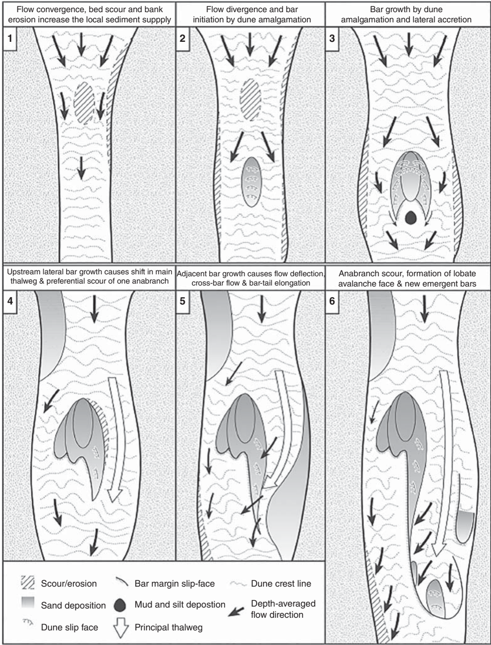
Figure 20.18 Summary model of the key stages in the evolution of a kilometre-scale mid-channel sand bar. Dune orientations and flow directions at the bed are inferred from the data presented in Roden (1998) and McLelland et al. (1999). Source: From Ashworth et al. (2000). © 2000, John Wiley & Sons.
