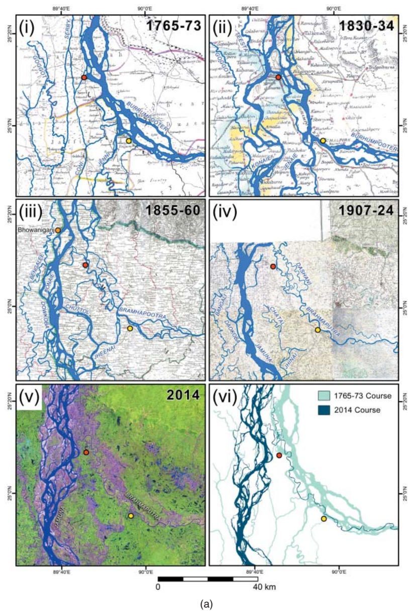
Figure 20.5 (a) Maps showing the avulsion of the Brahmaputra River into the contemporary course of the Jamuna. These maps illustrate the reduction in flow in the Brahmaputra River (Burrumpooter in (i), now called the Old Brahmaputra) and gradual establishment of an independent Jamuna braidbelt, with flow initially being diverted down the channels of the Konaie and Jenaie rivers (ii, iii). The avulsion was largely complete by 1855–60 (iii). The red and yellow dots show positions of the towns of Dewanganj and Jamalpur, respectively. Source: Modified from Bandyopadhyay et al. (2021). (b) Historical changes in the position of the bankline of the Jamuna River. Source: Based on EGIS (1997).
