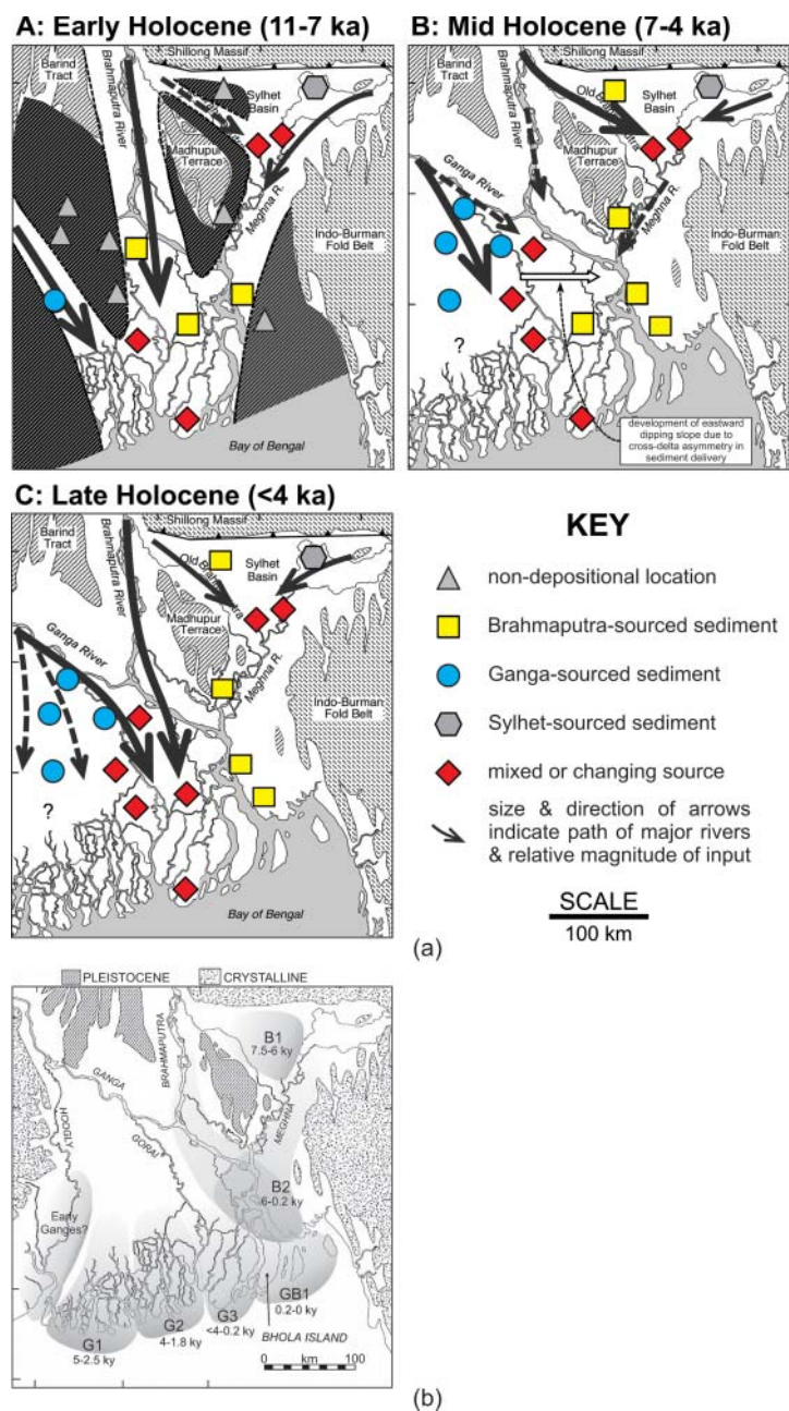
Figure 20.3 (a) Reconstruction of the principal river pathways and patterns of sediment distribution associated with the Ganga, Brahmaputra (Jamuna), and Sylhet sources through the Holocene. A: In the Early Holocene, rivers are constrained within their lowestland valleys, and there is limited influence of the Brahmaputra River in the Sylhet basin. B: In the Mid-Holocene, slower sea-level rise allows rivers to infill their valleys, which subsequently become more mobile across the delta. C: By the Late Holocene, the principal rivers interact on the central delta plain, shifting toward the present-day confluence and the estuary that receives discharge from all the rivers. Source: Modified from Goodbred et al. (2014). (b) Palaeogeographic reconstruction of the timing and location of river channel change and associated delta lobes during the Middle-Late Holocene. The delta lobes are associated with the Ganga (G1, G2, G3), Brahmaputra (B1, B2) and combined Ganga–Brahmaputra (GB1) river sources. Source: Modified from Akter et al. (2016).
