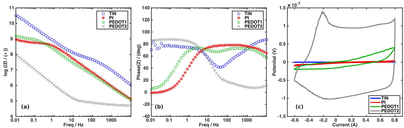
Fig. 6. (a,b) Bode plot ((a) amplitude and (b) phase) of impedance spectra of a TiN electrode, a Pt electrode and two PEDOT:PSS electrodes (deposited with PEDOT1 and PEDOT2 programs) (30 μm diameter). EIS at 1 kHz are equal to 9.32 MΩ, 875 kΩ, 720 kΩ and 58 kΩ for TiN, Pt, PEDOT1 and PEDOT2 electrodes, respectively. (c) CV measurement from four types of the microelectrodes combined in one graph.
