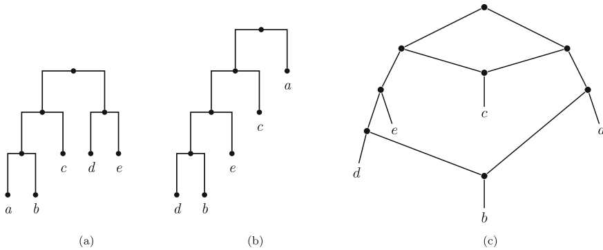
Fig. 1 The binary trees in (a) and (b) are both displayed by the network in (c)
