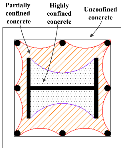
(a) H-shaped steel
