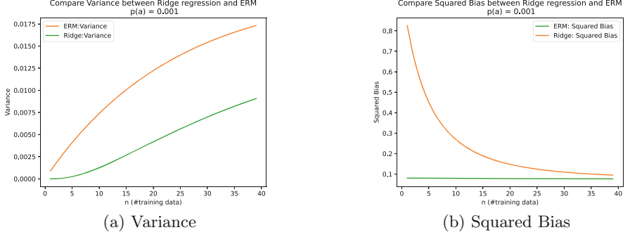
Fig. 3. Comparison of the variance and squared bias terms for ERM and ridge regression
