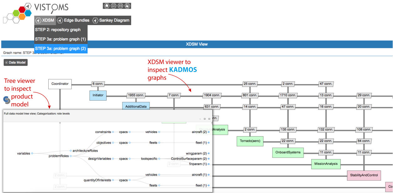
Fig. 8 Step IIIa: Screenshot of the web-based VISTOMS interface (C5) showing an XDSM visualization of the problem graph assembled by KADMOS (C4) and a tree view with some elements from the CPACS (C2) product model, with assigned problem roles.
