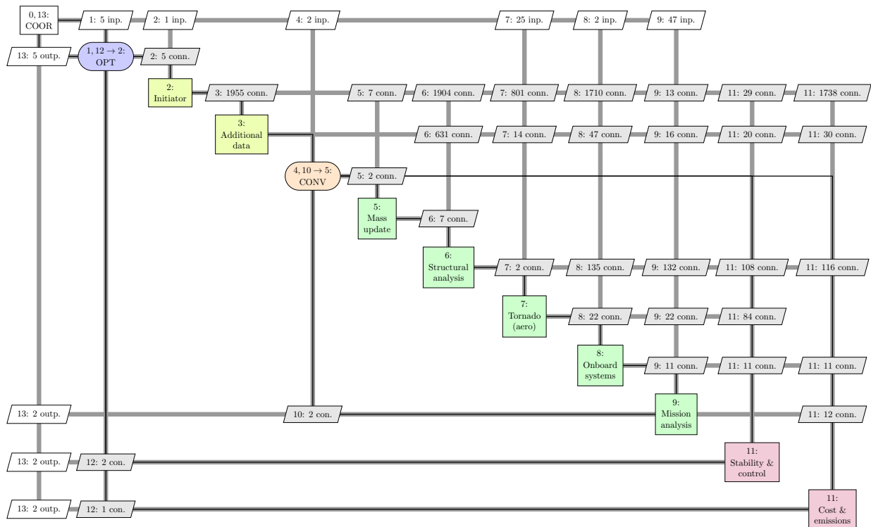
Fig. 9 Step IIIb: XDSM showing the MDO solution strategy formulated by KADMOS (C4) based on the MDF architecture. Same figure as BWA MDO snapshot in Figure 4.
