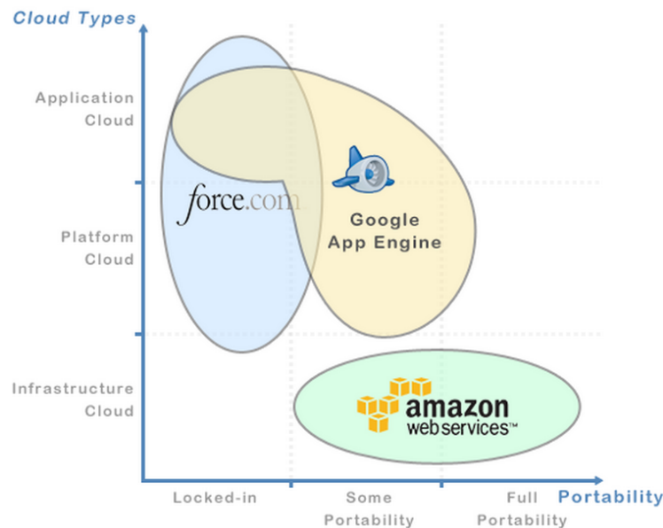
Figure 4.2: Cloud Portability
