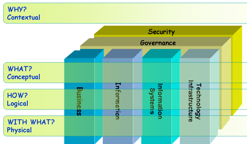
Figure 6.2: IAF Overview
