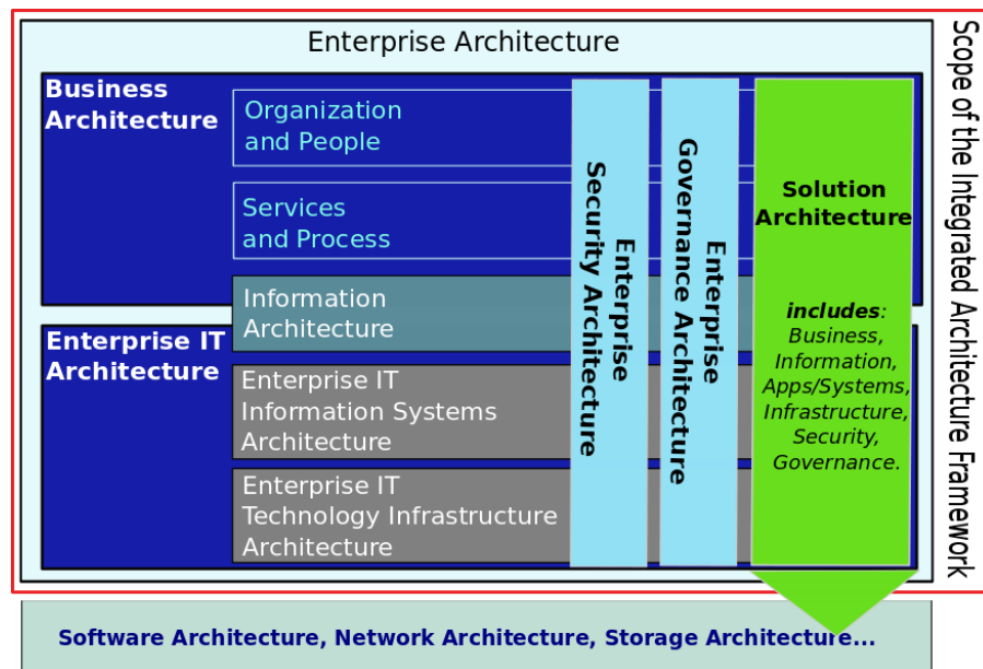
Figure 6.1: IAF Scope
