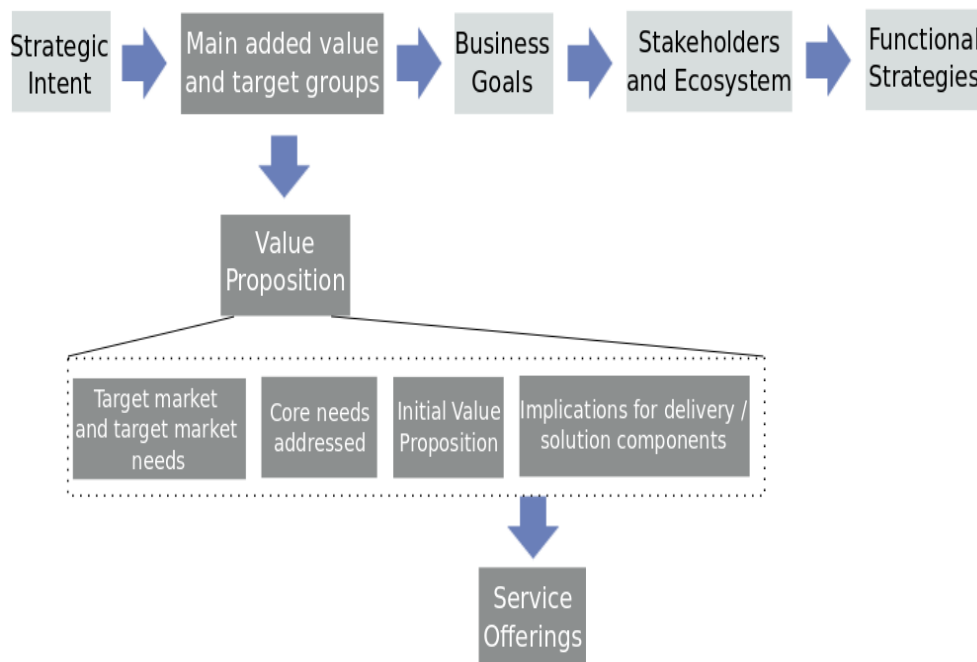
Figure 9.1: Value Proposition
