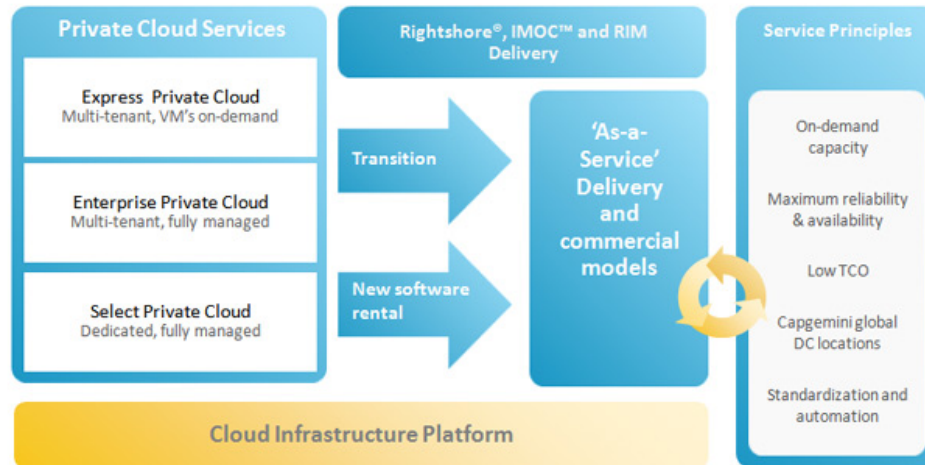
Figure 3.5: Capgemini IaaS
