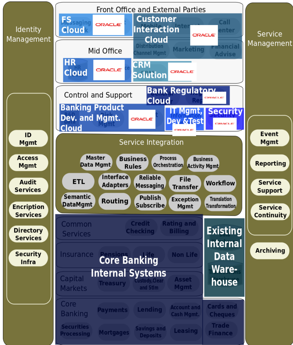
Figure 8.5: Final Architecture
