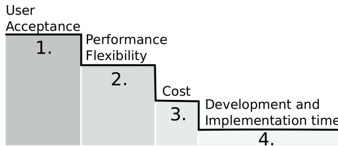
Figure 8.4: Knock-Out Criteria
