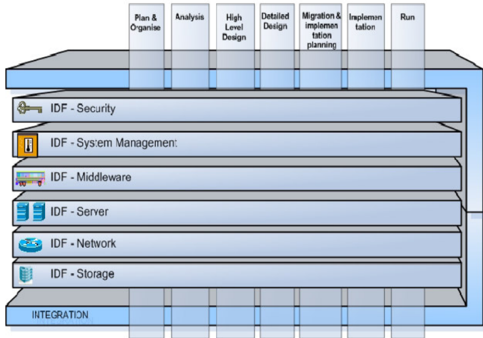
Figure 6.3: IDF Overview
