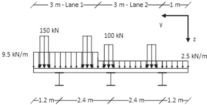
Fig. 6. Cross section of the generic bridge with loads
