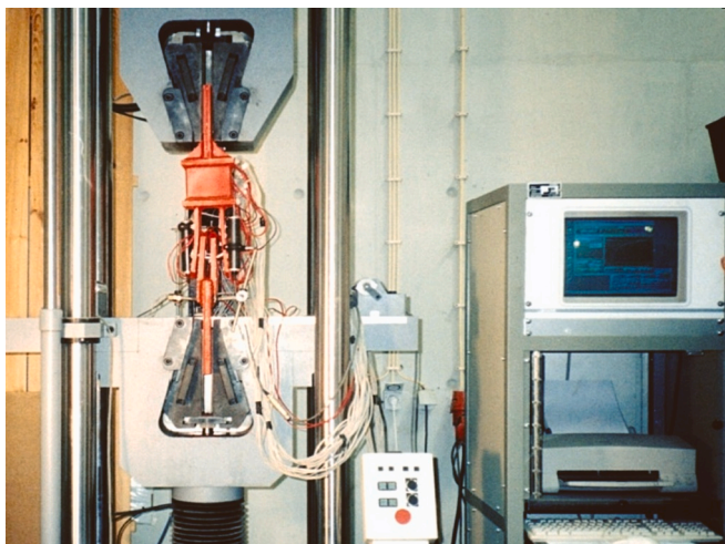
Fig. 9. Test setup.
