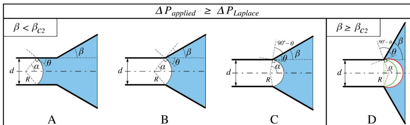
Figure 3. Forced retreating liquid meniscus due to increased applied gas pressure \Delta P_{\text{applied}} (applied from the left). A) Situation comparable to Figure 2A, where the meniscus is in straight-walled capillary and \alpha = 90^\circ - \theta . B) \alpha remains the same as in (1) unless \Delta P_{\text{applied}} is increased. C) When \Delta P_{\text{applied}} is increased, the meniscus changes its curvature and \alpha is defined as \alpha = 90^\circ - \theta + \beta . D) For angles \beta \geq \beta_{c2} , the meniscus will progress through its minimal radius R causing the burst pressure to reach its maximum, \Delta P_{\text{burst}} = \frac{4\gamma}{d} .
