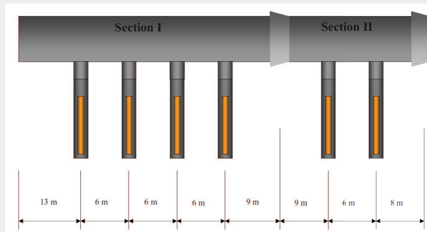
Figure 2.6: Layout of the prototype repository simulation (Dahlström, 2009).
