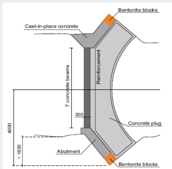
Figure 2.5: The plug design of the backfill and plug test (Malm, 2012).
