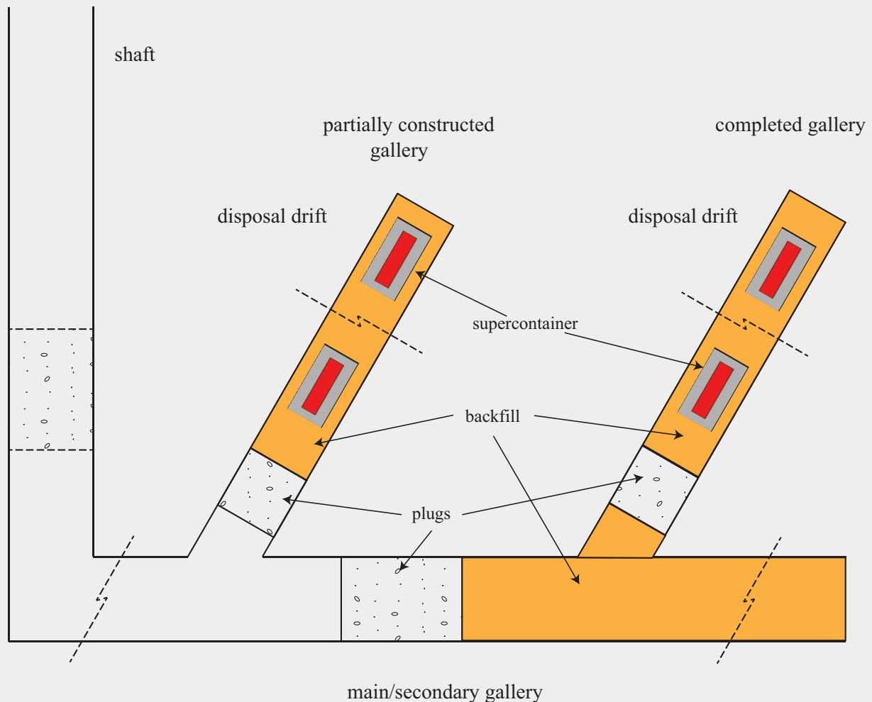
Figure 3.1: Schematic layout of plug locations in the repository concept. Main and secondary galleries are horizontal and the shaft is vertical.
