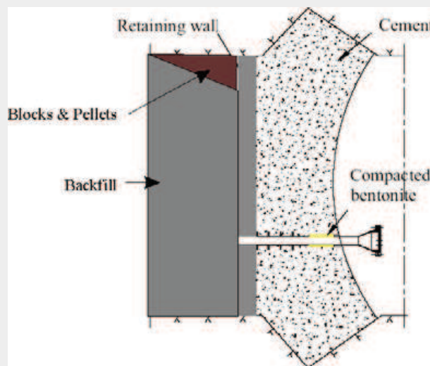
Figure 2.7: Design of the dome shape plug used in the prototype repository (Johannesson et al., 2004).
