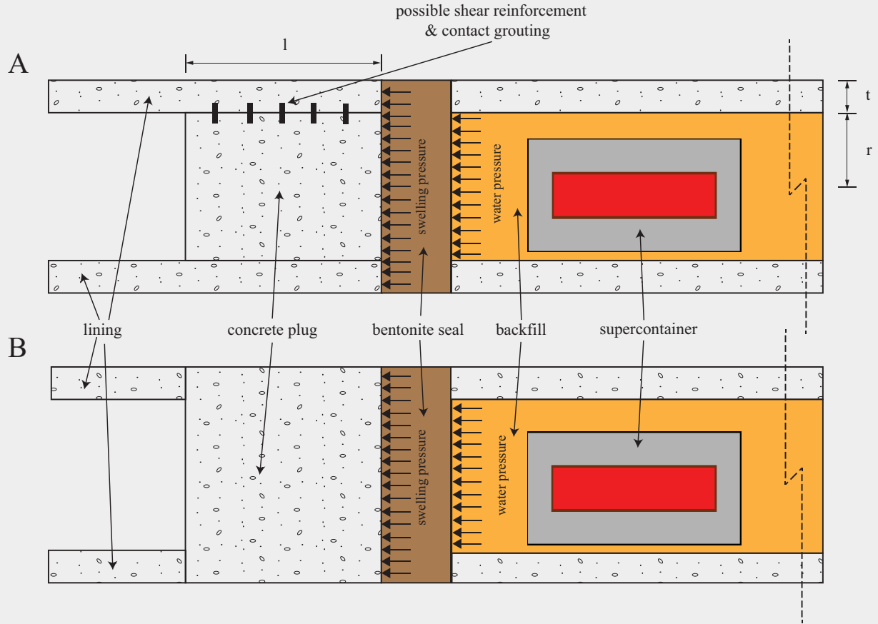
Figure 3.2: Two types of conceptual plug design, (A) with the concrete plug installed inside the tunnel lining, and (B) with the tunnel lining removed locally where the concrete plug is installed.
