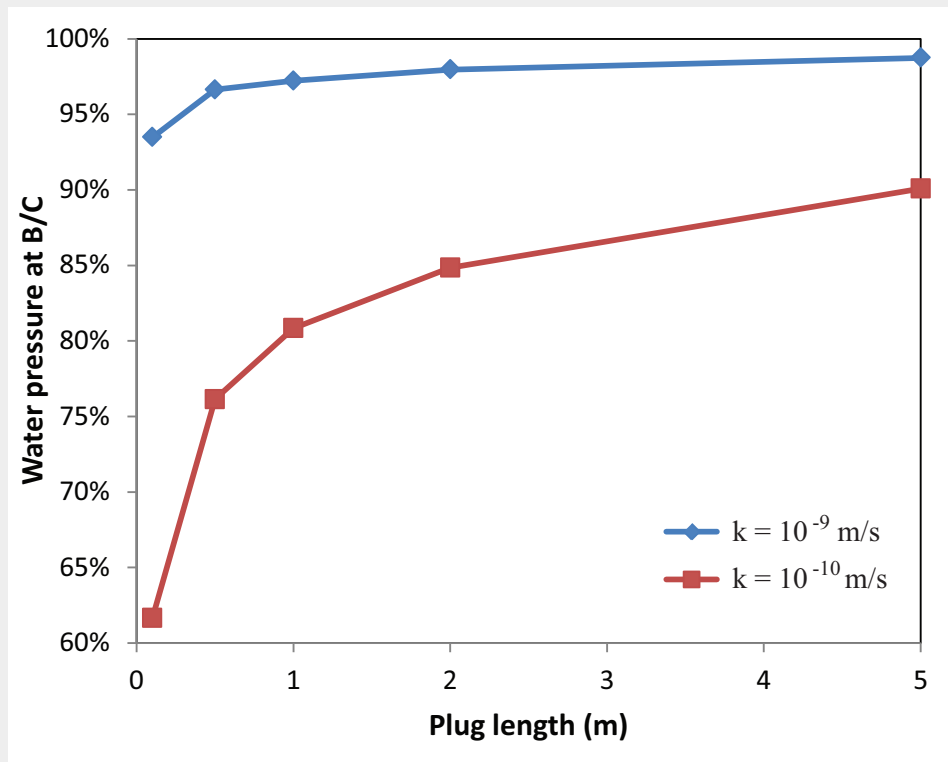
Figure 3.6: Percentage of water head taken by the plug versus sealing length, for different backfill hydraulic conductivities
