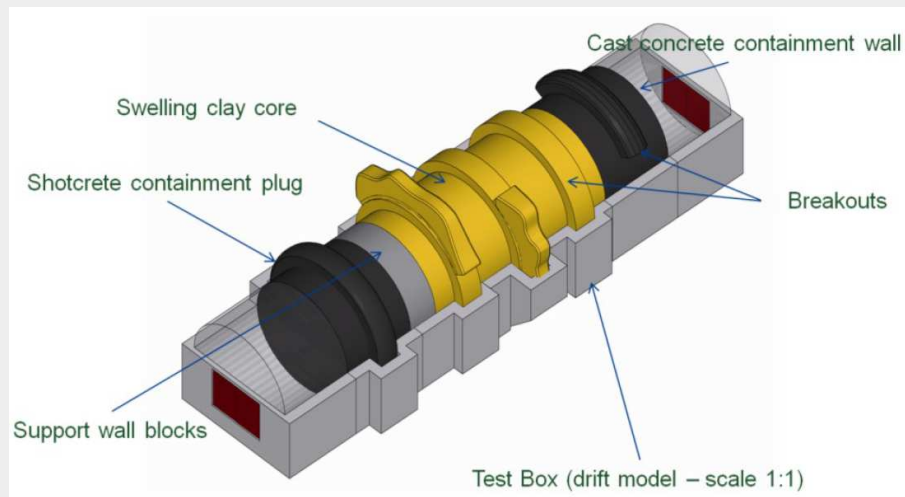
Figure 2.13: Layout of the FSS conceptual design (White et al., 2014).
