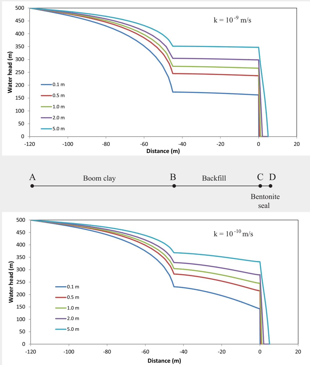
Figure 3.5: Pore pressure head distribution along the tunnel for different sealing lengths, top: k=10^{-9} \text{ m/s} for the backfill hydraulic conductivity; bottom: k=10^{-10} \text{ m/s} for the backfill hydraulic conductivity.
