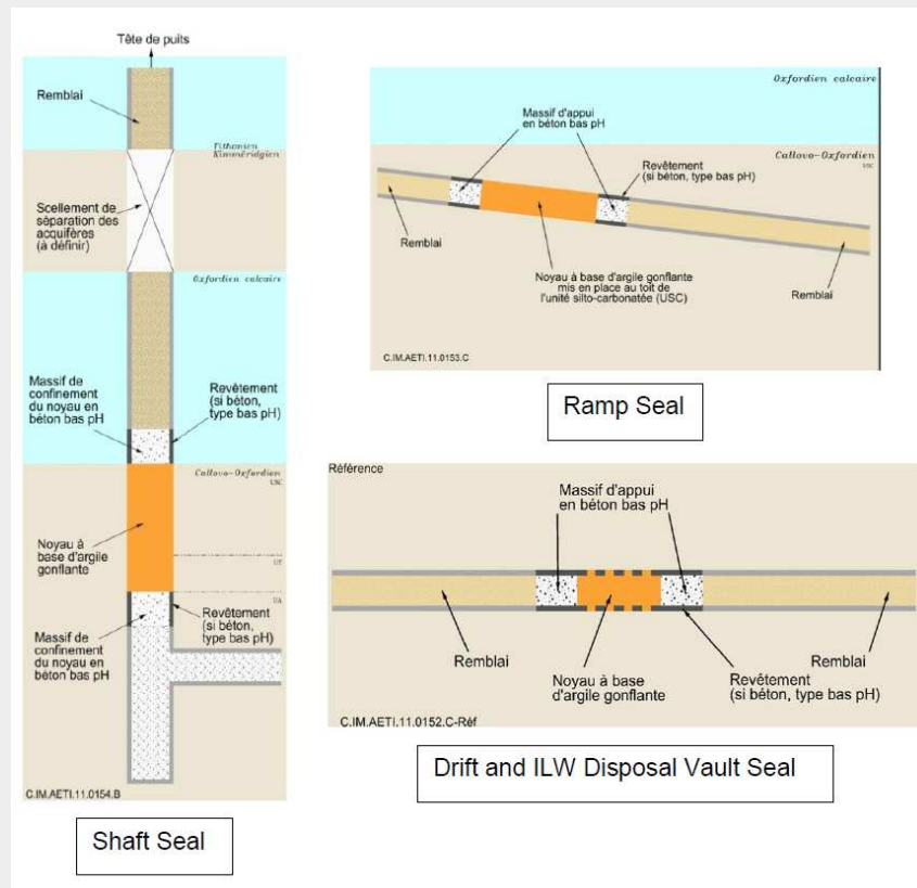
Figure 2.12: Conceptual designs for each type of seal (White et al., 2014).
