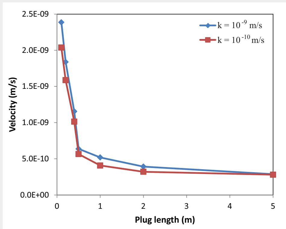
Figure 3.7: Maximum velocity in the domain versus sealing length for different backfill hydraulic conductivity (note: results for thicknesses of 0.2 and 0.4 m added for clarity).
