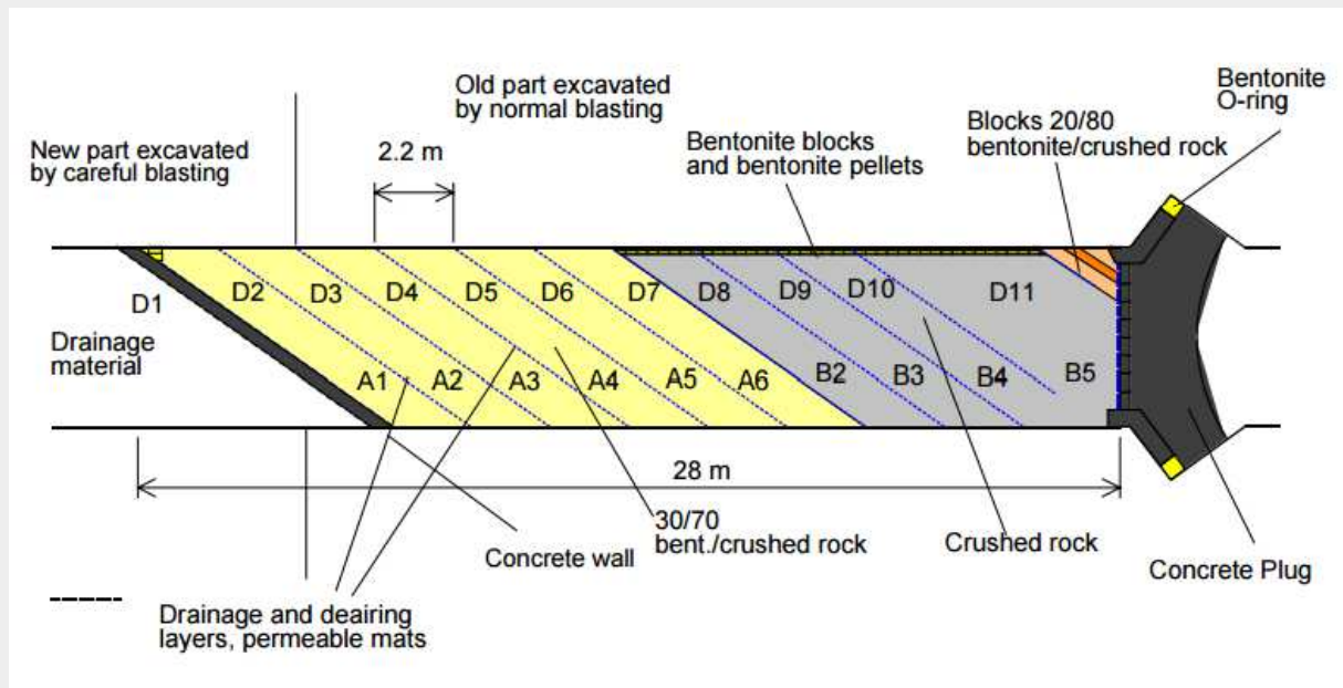
Figure 2.4: Layout of the backfill and plug test (Gunnarsson et al., 2001).
