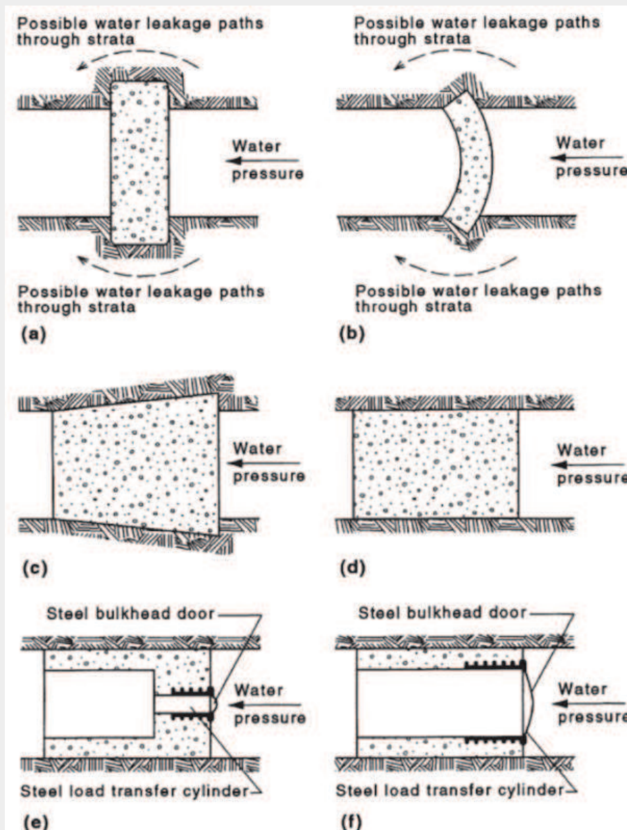
Figure 2.1: Generic plug shapes (Auld, 1983). (a) Reinforced concrete slab; (b) Unreinforced concrete arch; (c) Unreinforced concrete tapered plug; (d) Unreinforced concrete parallel plug; (e) Unreinforced concrete cylindrical parallel plug, with human access; (f) unreinforced concrete cylindrical parallel plug, with roadway access.
