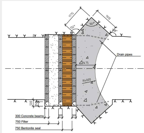
Figure 2.8: Layout of the KBS-3V reference plug design (Malm, 2012).
