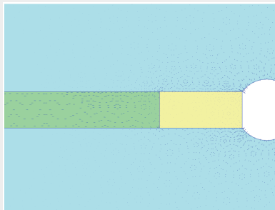
Figure 3.8: Velocity distribution near the plug for different sealing lengths, left: k=10^{-9} m/s for the backfill hydraulic conductivity; right: k=10^{-10} m/s for the backfill hydraulic conductivity.
