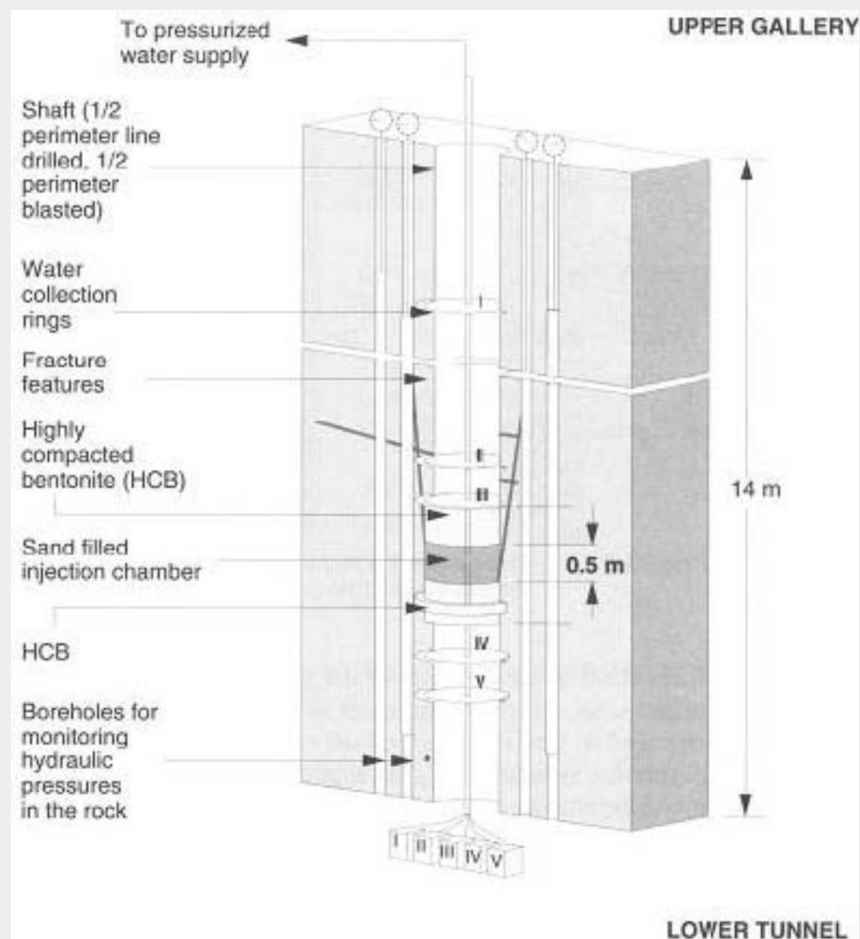
Figure 2.3: Design of the Shaft Sealing Test (Gray, 1993; Pusch et al., 1987a).
