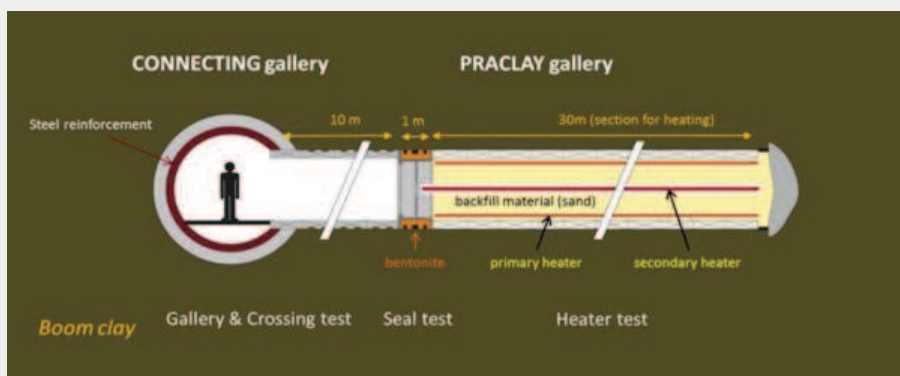
Figure 2.11: Layout of the PRACLAY experiment (Van Marcke et al., 2013).
