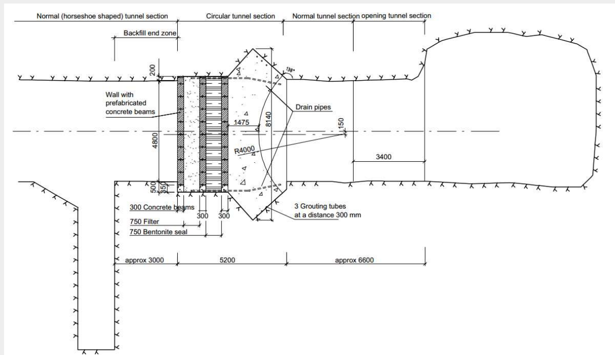
Figure 2.9: Schematic view of the KBS-3V reference plug system (Malm, 2012).
