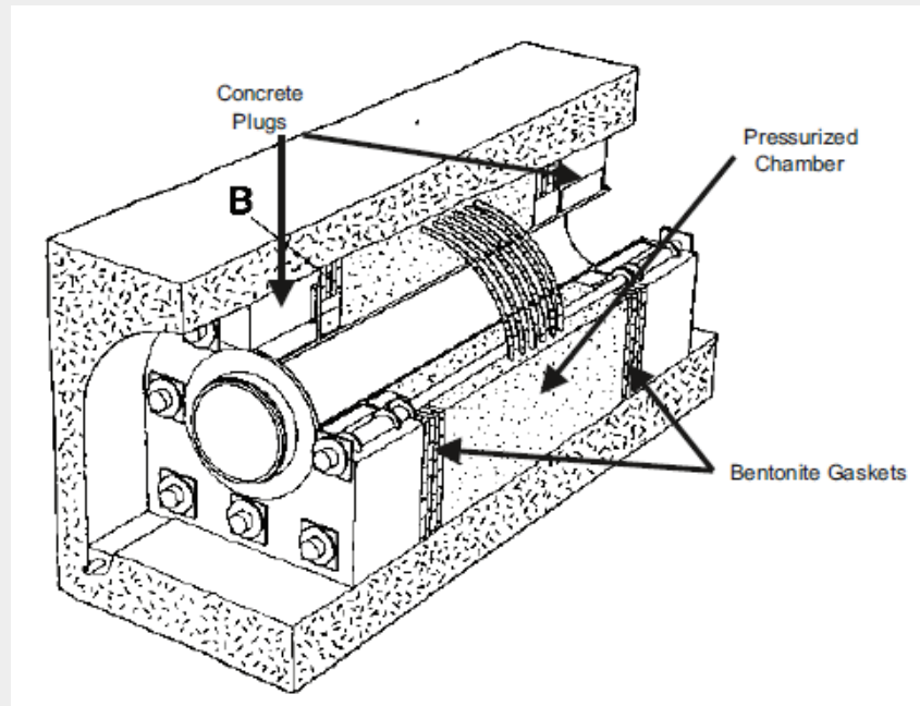
Figure 2.2: Design of the tunnel plugging experiment (Pusch et al., 1987b).
