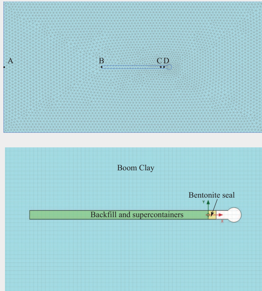
Figure 3.3: The mesh and details of the deposition tunnel and plug system used for the hydraulic simulation.
