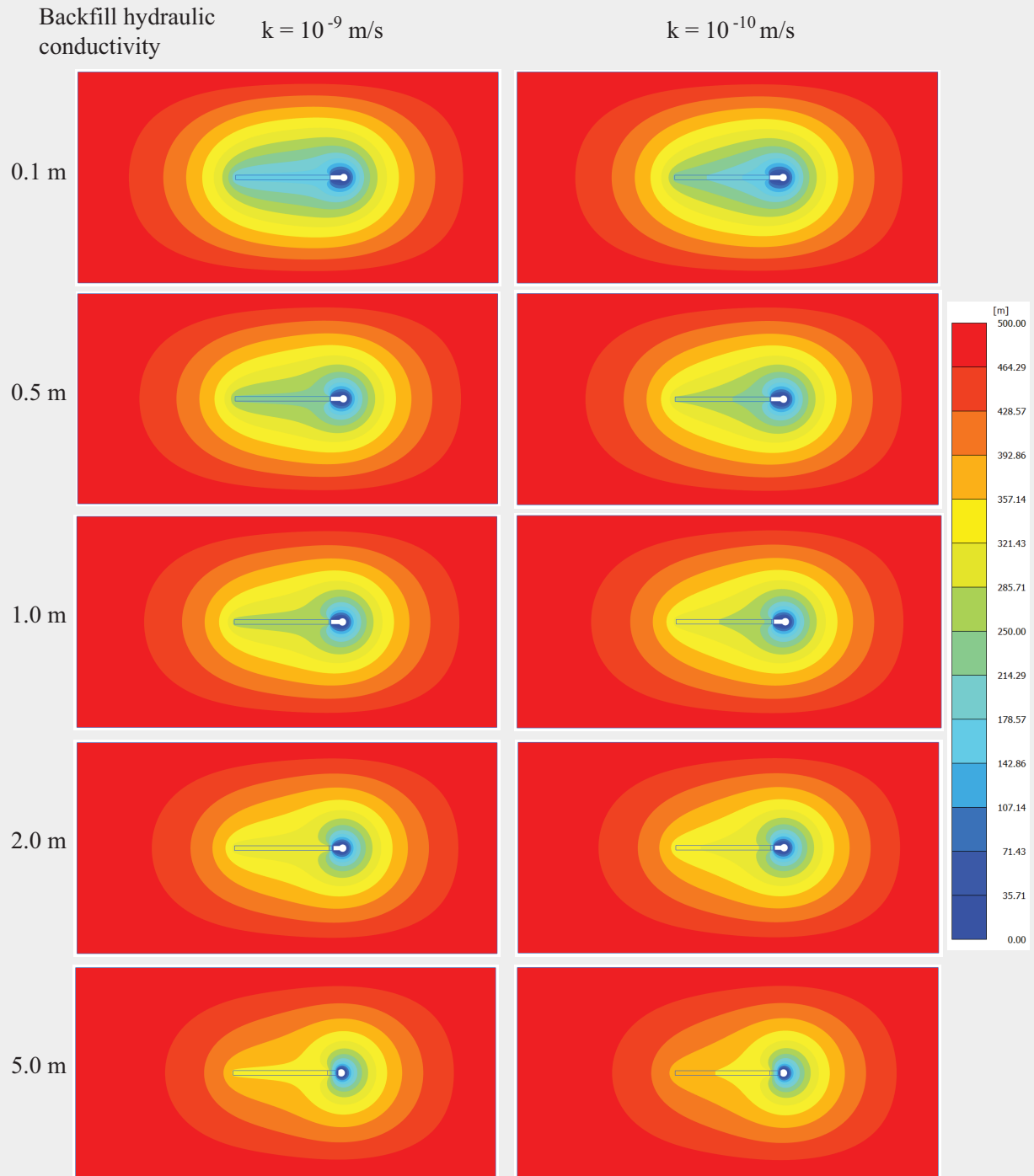
Figure 3.4: Pore pressure head distribution for different sealing lengths, left: k=10^{-9} m/s for the backfill hydraulic conductivity; right: k=10^{-10} m/s for the backfill hydraulic conductivity.
