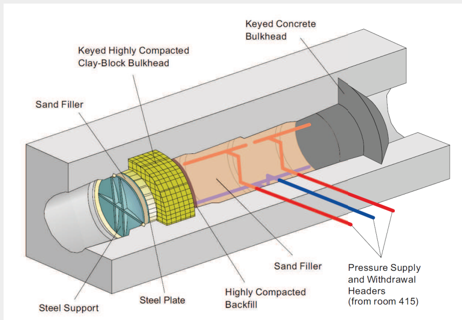
Figure 2.10: Layout of the tunnel sealing experiment (Chandler et al., 2002).
